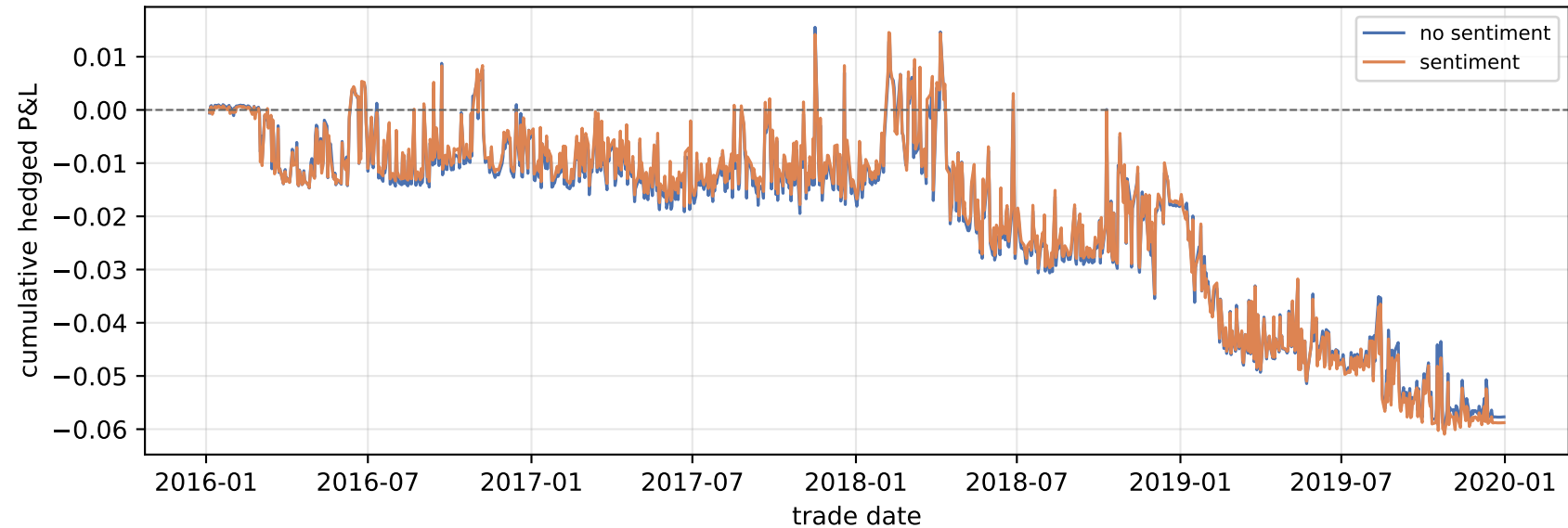
Delta-hedged P&L — Bergomi 2016-2019 variance NS 3.36\text{e-}05 | S 3.20\text{e-}05
