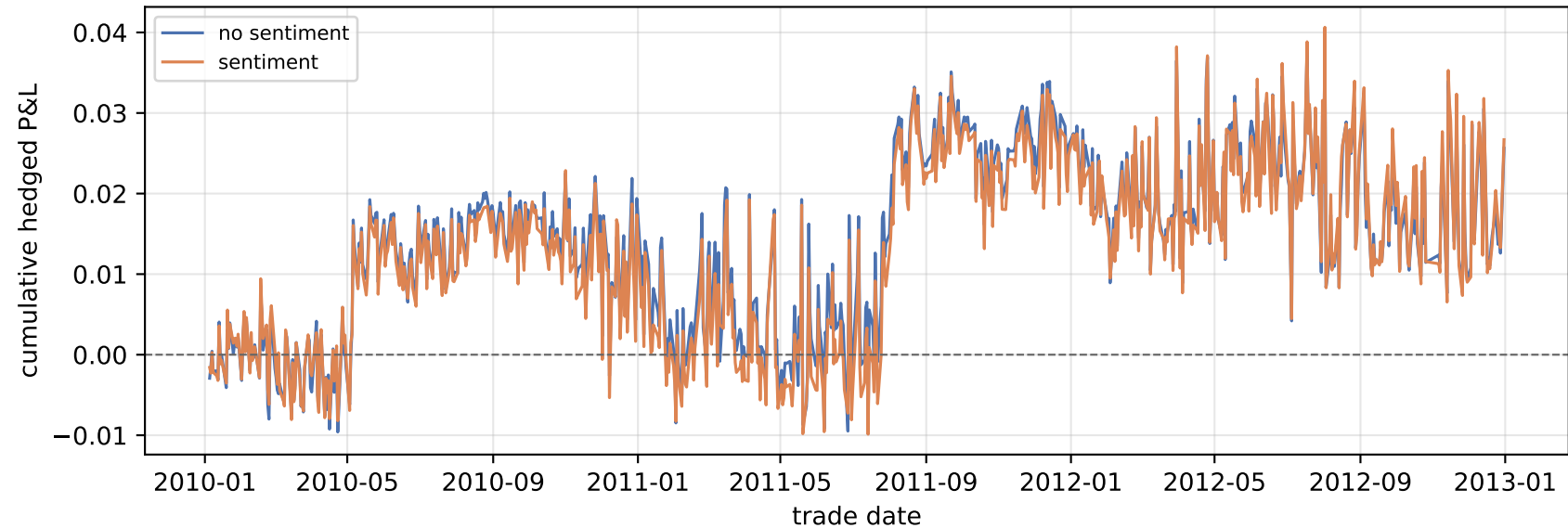
Delta-hedged P&L — rBergomi 2010-2012 variance NS 4.39\text{e-}05 | S 4.86\text{e-}05
