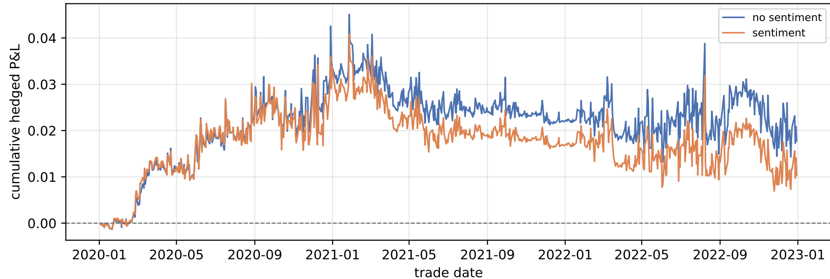
Delta-hedged P&L — rBergomi 2020-2022 variance NS 1.11\text{e-}05 | S 9.32\text{e-}06
