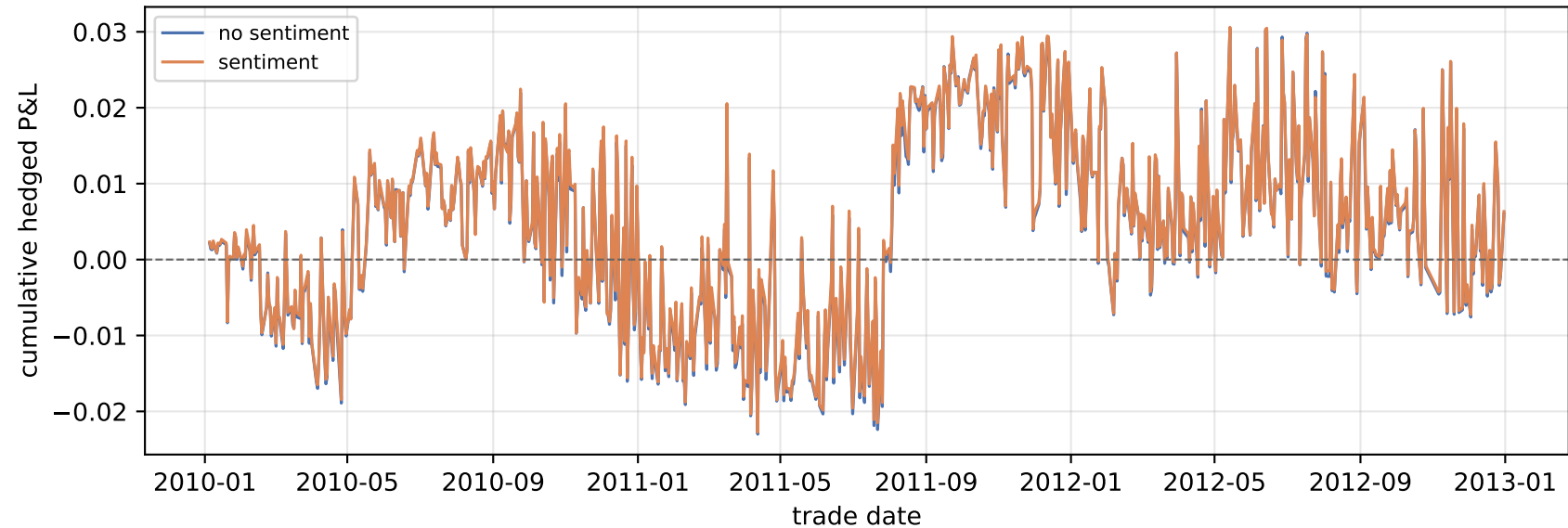
Delta-hedged P&L — Bates 2010-2012 variance NS 8.25e-05 | S 8.22e-05
