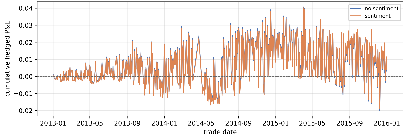
Delta-hedged P&L — Bates 2013-2015 variance NS 1.54e-04 | S 1.52e-04
