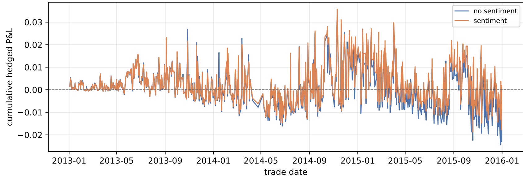
Delta-hedged P&L — Bergomi 2013-2015 variance NS 9.56e-05 | S 8.93e-05
