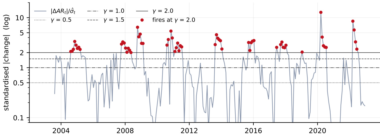
Standardised absorption-ratio change and trigger thresholds
