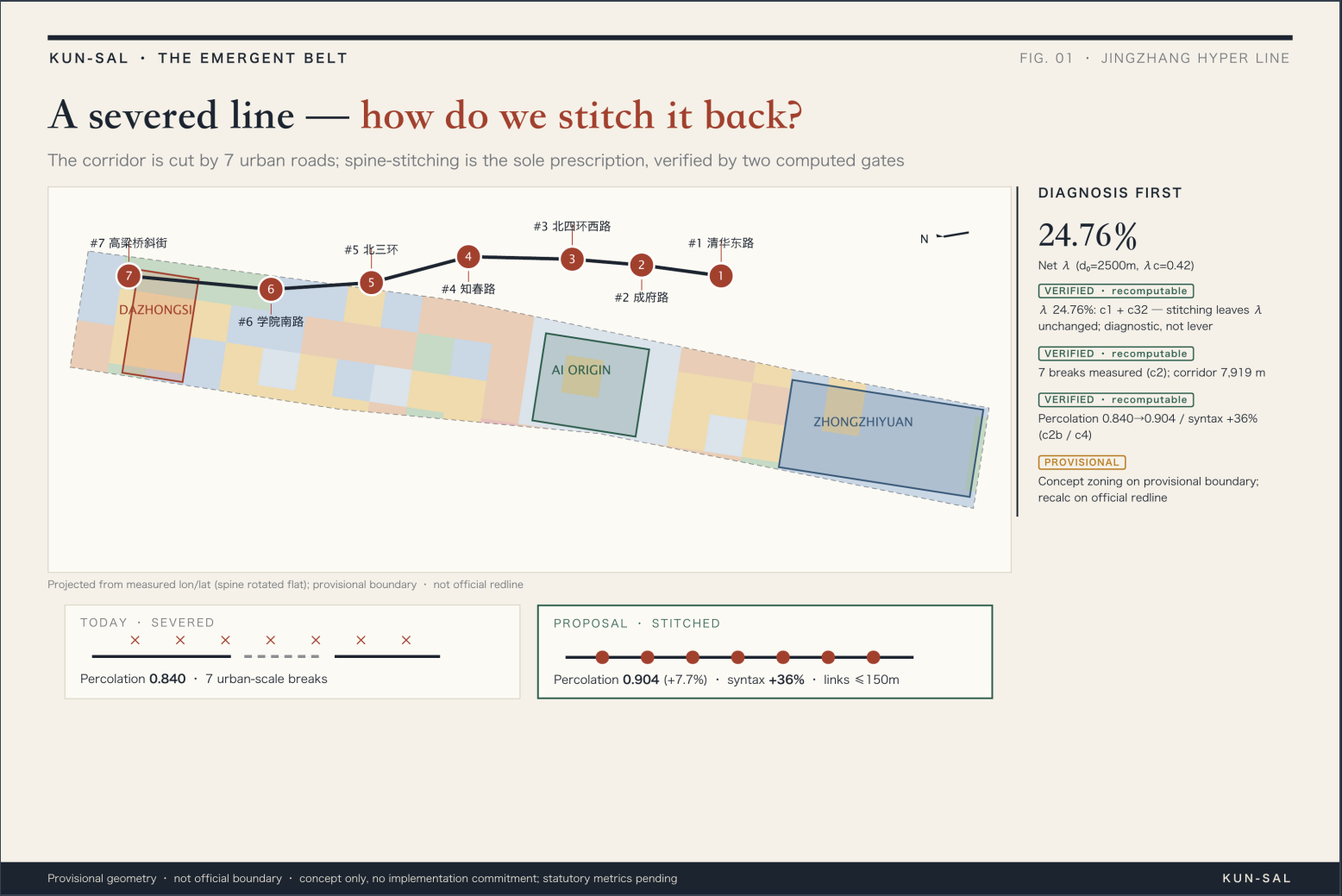
FIG.01 · severance diagnosis & spine stitching (measured geometry)
