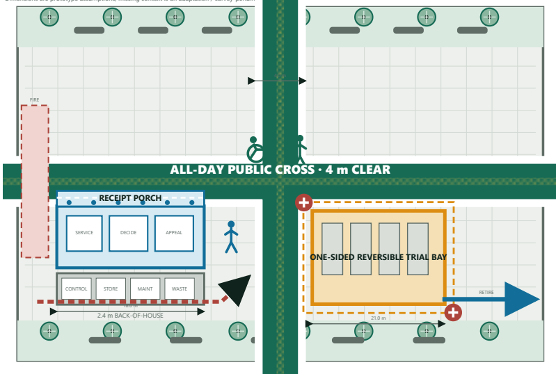
DAZHONGSI BUILDABLE CIVIC CROSS · 1:500 ARCHITECTURE + GROUND PLAN
