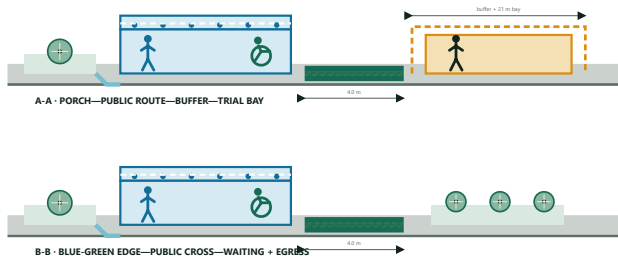
TWO 1:200 SECTIONS · PUBLIC BASELINE + PLUG-IN HAVE A LEGIBLE PHYSICAL EDGE
