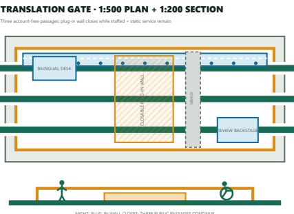
TRANSLATION GATE · 1:500 PLAN + 1:200 SECTION
