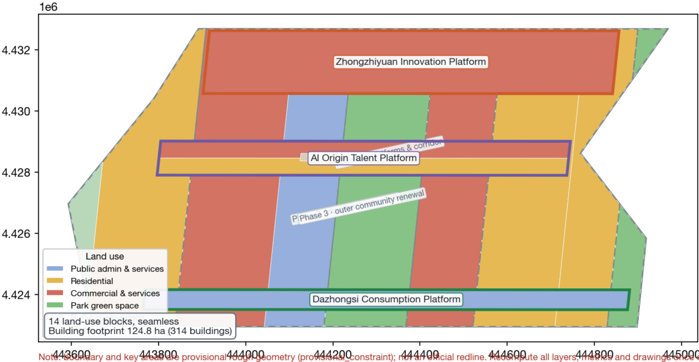
Land-use structure, phasing, and retain-renoate-demolish strategy · 用地结构、分期与拆改留方案
