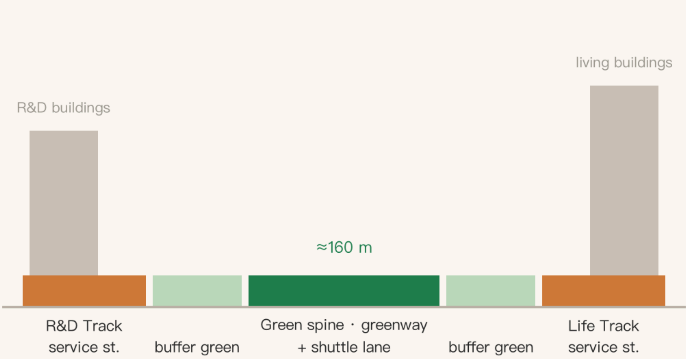
Spine standard section (conceptual)
