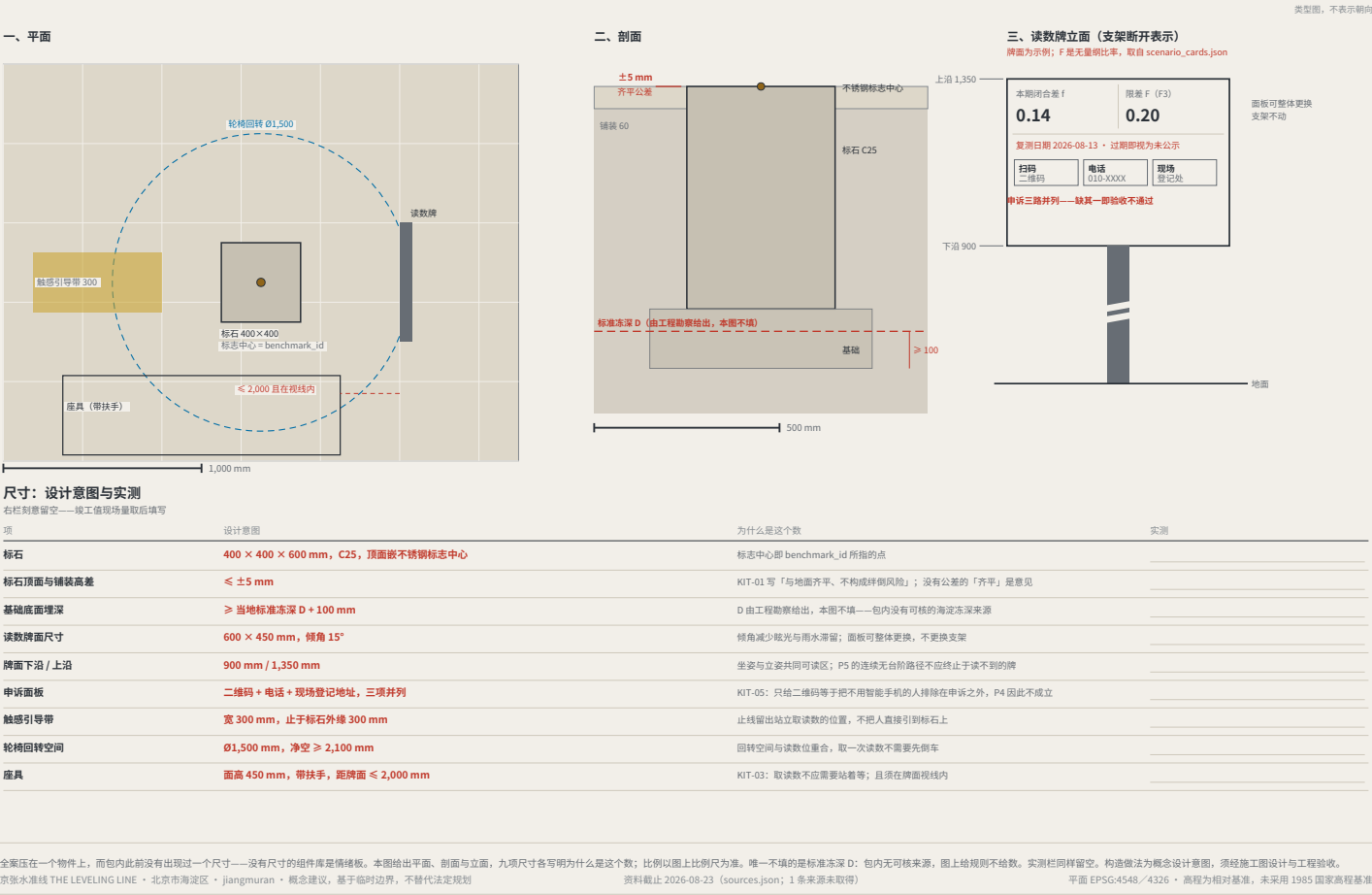
FIG.16 The benchmark and its reading plate, as a construction detail
