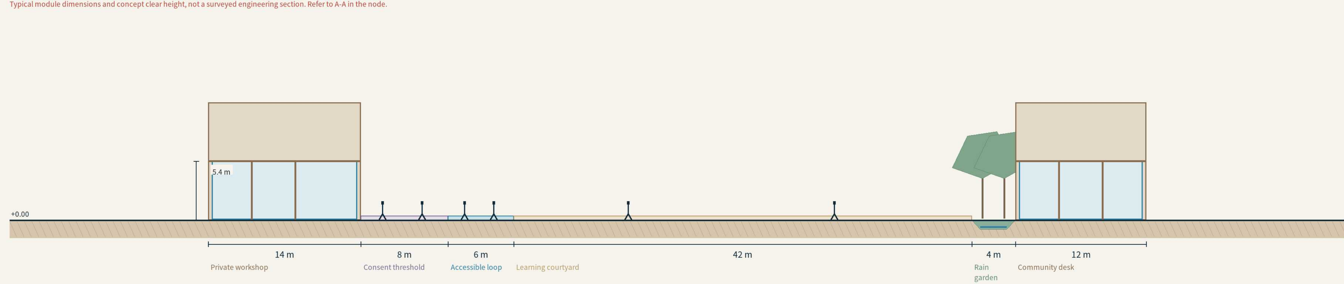
04 A-A Campus, park and community interface | 1:200 Typical module dimensions and concept clear height, not a surveyed engineering section. Refer to A-A in the node.
