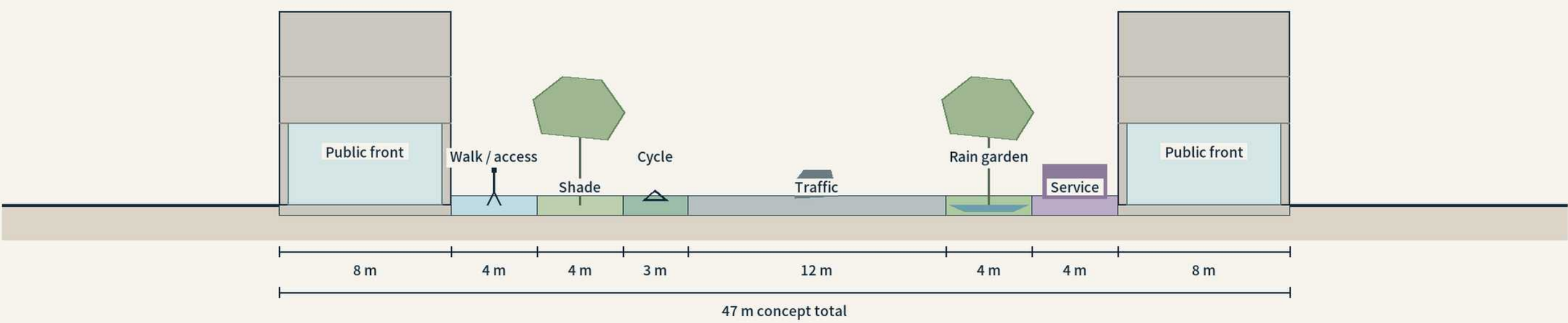
S2 Street and crossing edge | R03-03
