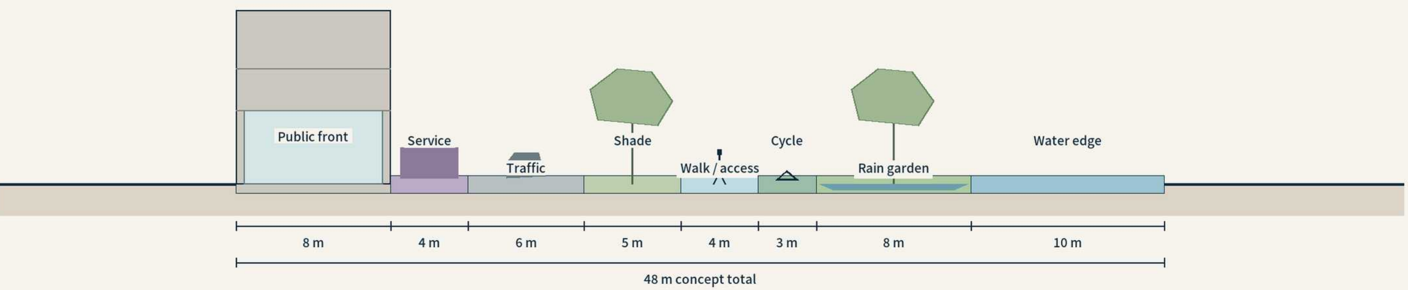
S3 Riverside blue-green buffer | R03-06
