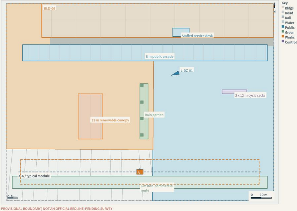
03 Provisional-area public ground | 1:500
