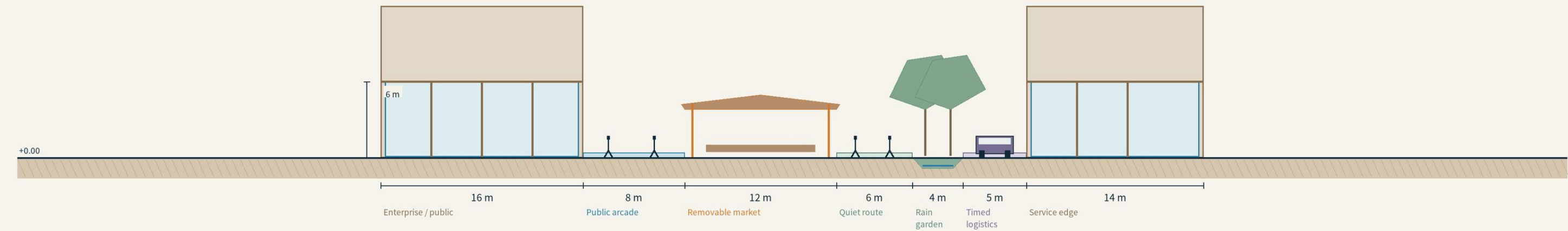
04 A-A Conditional transit, street and public ground | 1:200
