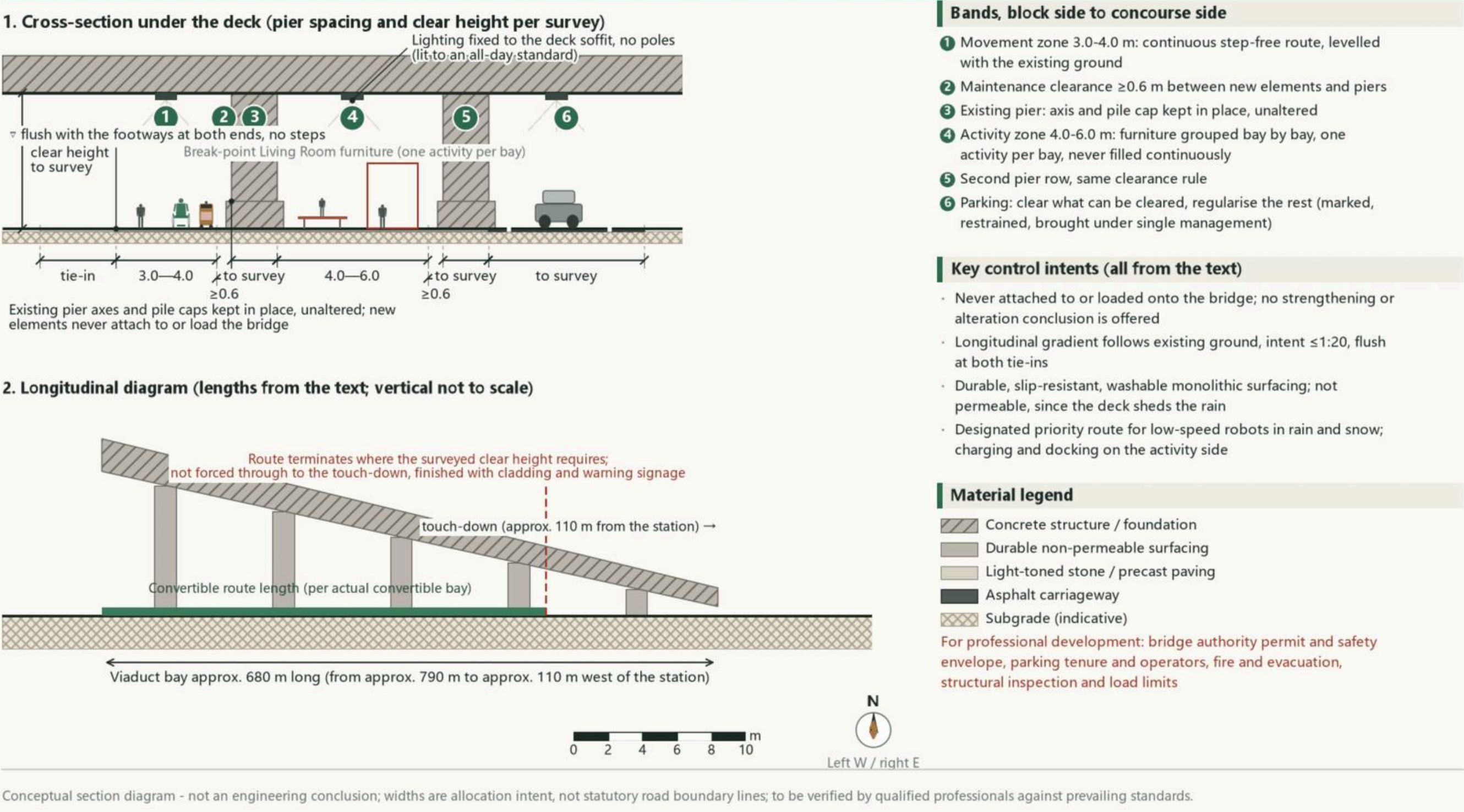
Section DZS-3: under-bridge space from ad-hoc parking to public use
