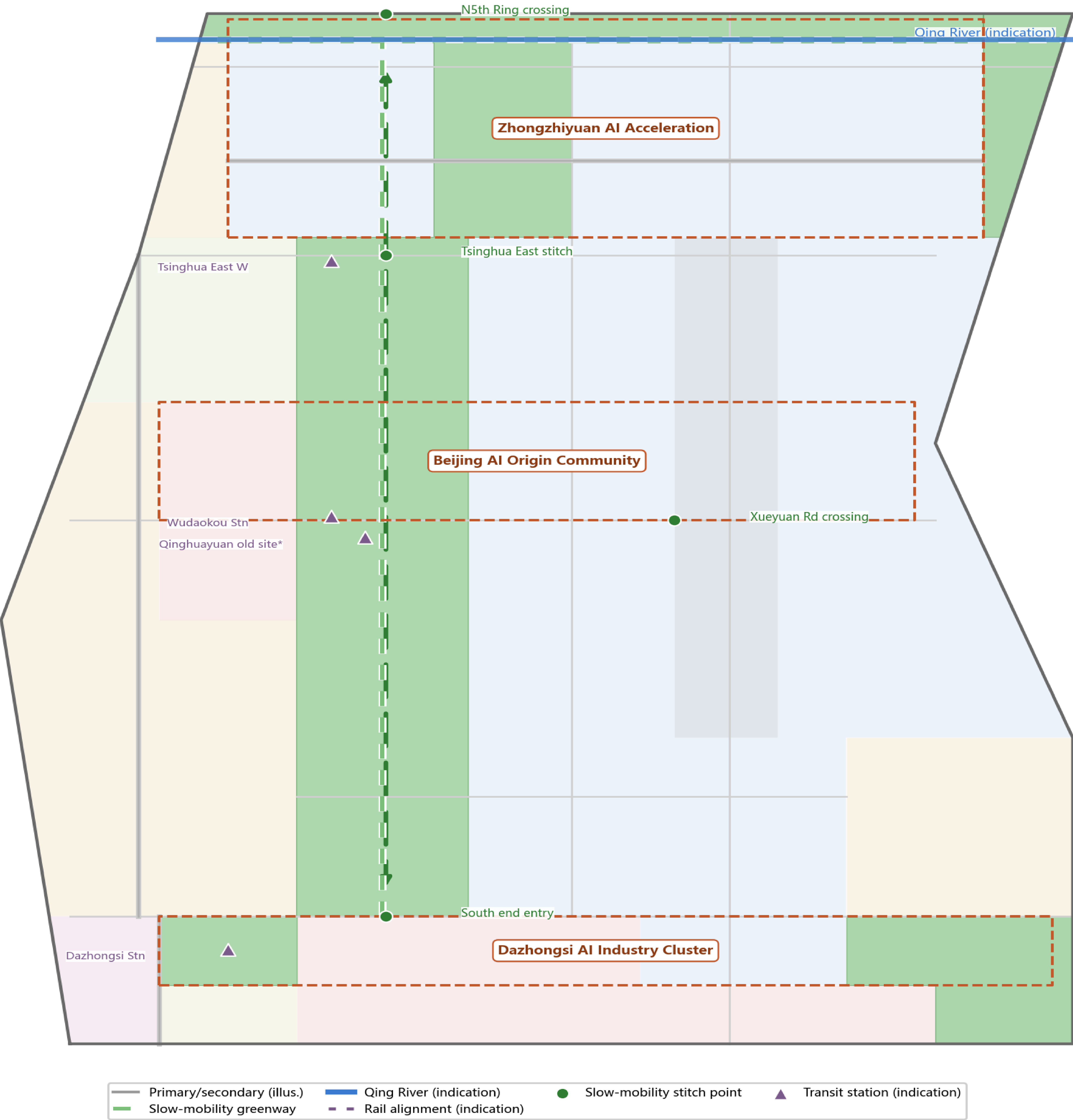
Fig 4: Slow-mobility greenway, Qing River frontage, stitch points, transit-station integration; road length 40.7 km (EPSG:4548); alignments are provisional.
