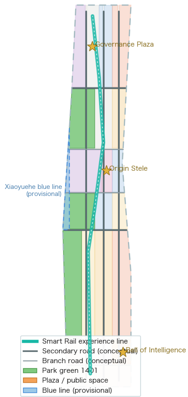
Fig.4 Mobility & Blue-Green Network · Smart Rail Line · Green · Public Space
