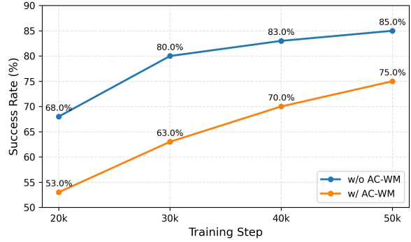
Figure 5: Success rates at different training steps in the AC-WM ablation study.
