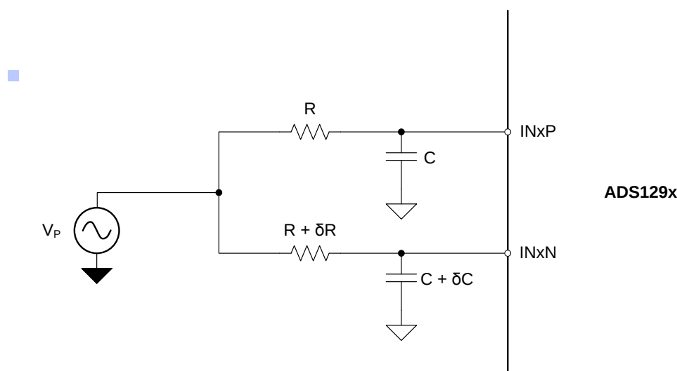
Figure 96. Typical Front-End Configuration
