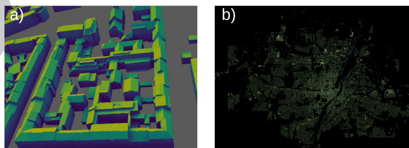
Figure 2: a) 3D mesh output of the CLI for a single Munich tile, with per-triangle annual PV yield mapped onto the building geometry (dark blue = low, light yellow = high). b) Orthographic top-down snapshots generated by the CLI for all Munich tiles, combined in one image.
