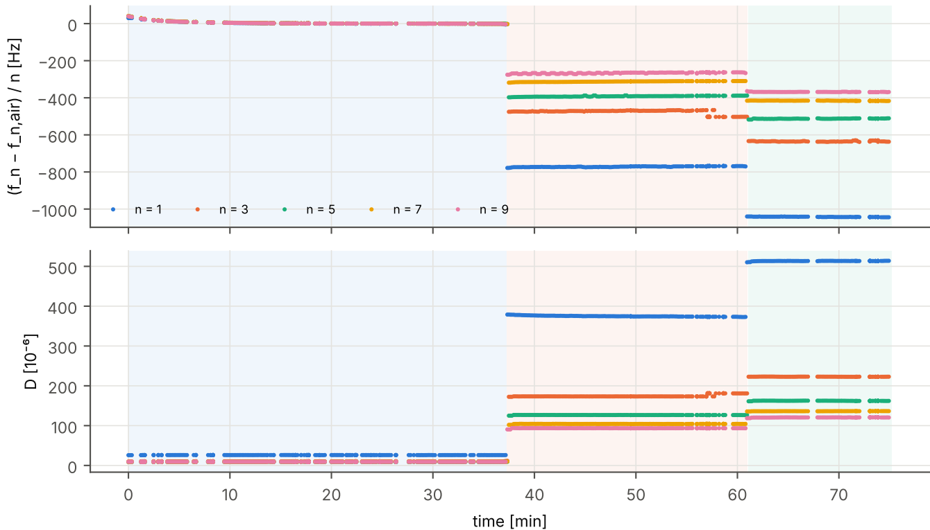
Run 2026-09-11: air \rightarrow water \rightarrow isopropanol, instrument datalog (max of G, half-height \Gamma )
