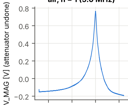
air, n = 1 (5.0 MHz)
