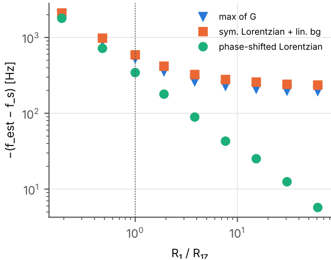
board phase \varphi_b = -20^\circ on H; \Gamma = 1 kHz
