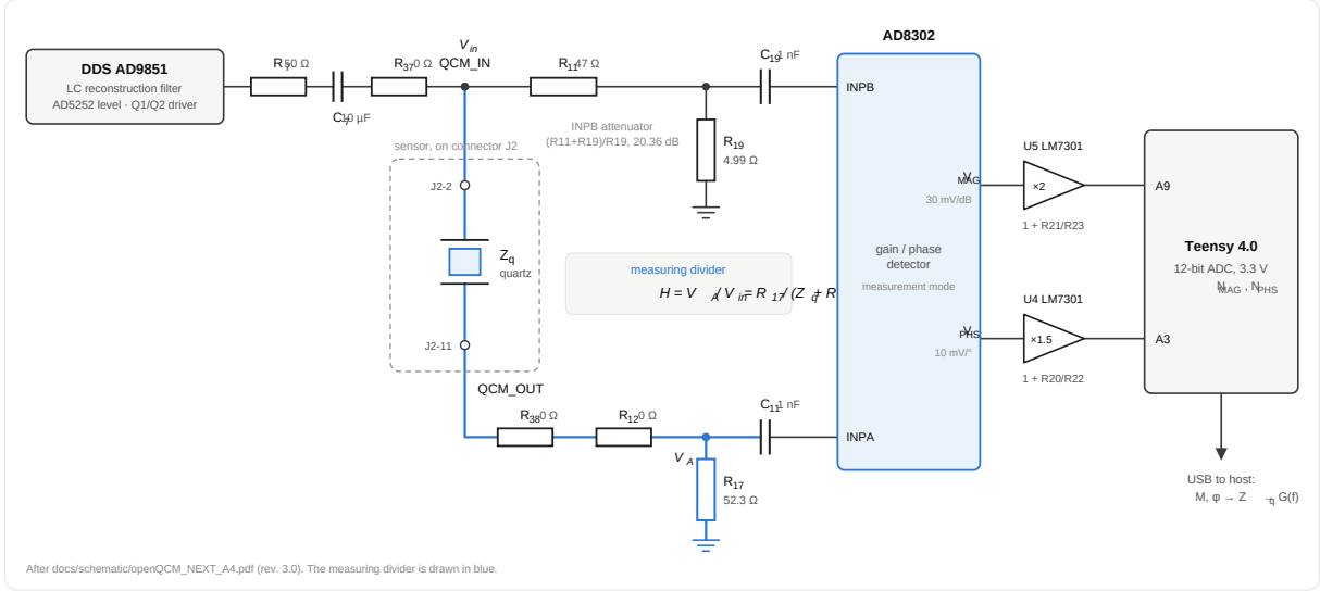
Figure 1: Measurement circuit: the quartz sensor in a divider with R_{17} , read by the AD8302 gain/phase detector; drawn after the openQCM NEXT schematic (repository figure).
