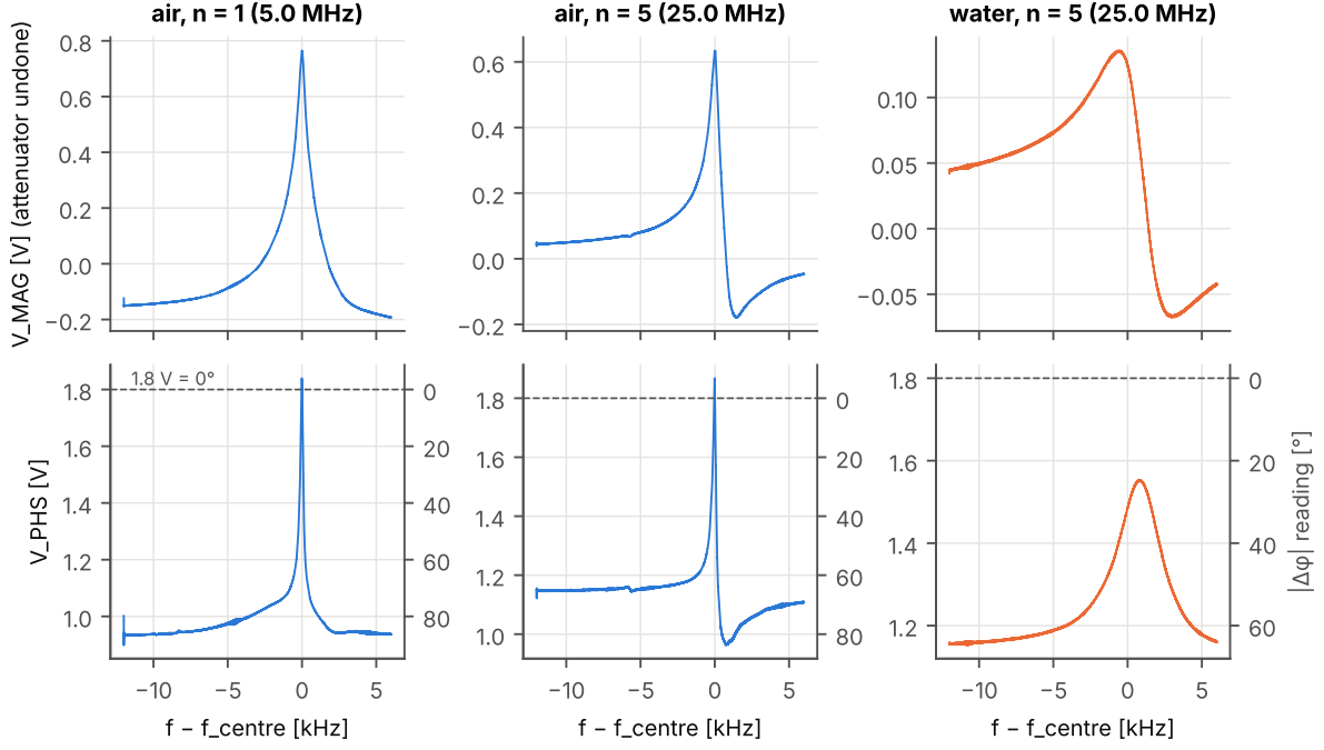
Figure 2: Raw detector voltages for the fundamental and the 5th overtone in air and for the 5th overtone in water (board 1920, 2026-09-11). Right axis: the unsigned phase reading |\Delta\phi| = (1.8 \text{ V} - V_{\text{PHS}})/10 \text{ mV} . In air the reading folds at zero (and overshoots it, the signature of the offset \delta ); in water it does not reach zero.
