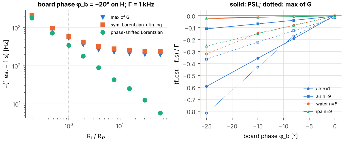
Figure 9: Forward model. Left: error of three estimators against R_1/R_{17} for a board phase of -20^\circ on the transfer function ( \Gamma = 1 kHz). Right: error in units of \Gamma against the board phase for four measured-like cases; solid: phase-shifted fit; dotted: maximum of G .
