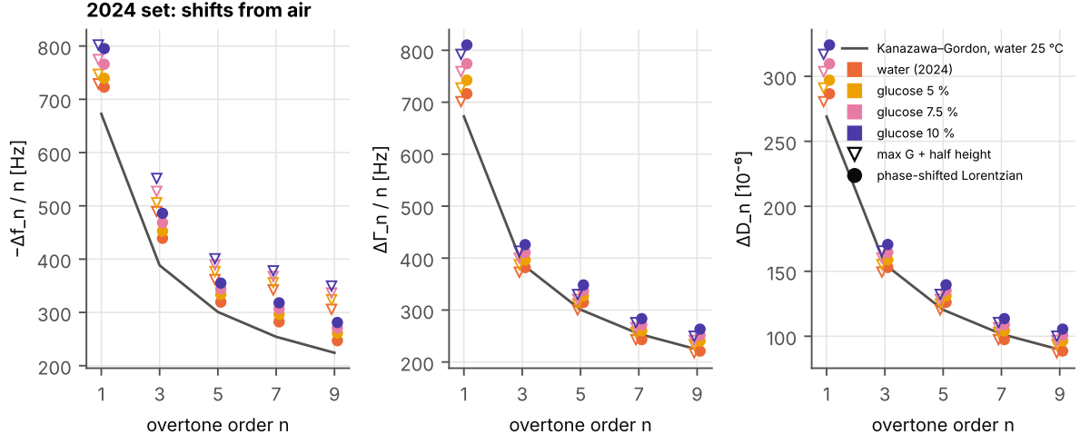
Figure 12: Second instrument: overtone-normalised shifts from air, -\Delta f_n/n , \Delta \Gamma_n/n and \Delta D_n , for water and the three glucose solutions, with the maximum of G (open triangles) and the phase-shifted Lorentzian (filled circles) and the Kanazawa–Gordon prediction for water.
