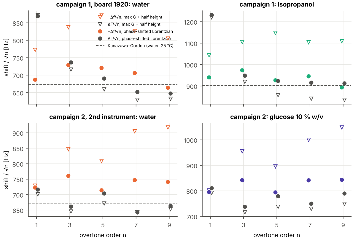
Figure 14: Overtone-normalised shifts -\Delta f_n/\sqrt{n} (coloured) and \Delta\Gamma_n/\sqrt{n} (grey) against the overtone order for the two campaigns, with the maximum of G (open triangles) and the phase-shifted Lorentzian (filled circles); a Newtonian liquid gives one horizontal line for both quantities, drawn for water at 25 °C.
