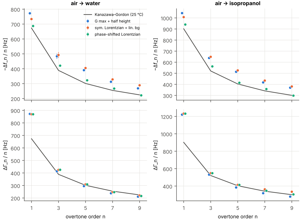
Figure 7: Overtone-normalised shifts -\Delta f_n/n (top) and \Delta \Gamma_n/n (bottom) against the overtone order for the maximum of G , the symmetric Lorentzian with linear background and the phase-shifted Lorentzian, with the Kanazawa-Gordon prediction at 25 °C. Error bars (mostly within the markers) are the replica scatter divided by n .
