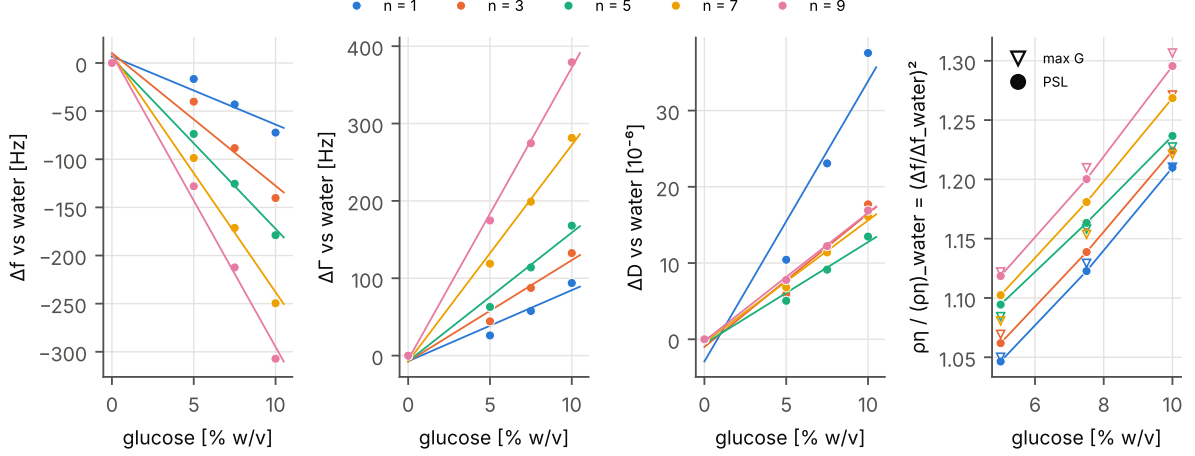
Figure 15: Second instrument: shifts relative to water of the fitted resonance frequency, half-bandwidth and dissipation against glucose concentration, one line per overtone (ordinary least squares with intercept), and the ratio \rho\eta/(\rho\eta)_{\text{water}} from the air-referenced frequency shifts with the two estimators.
