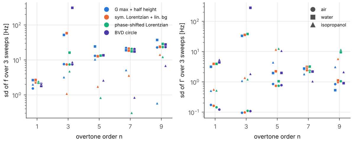
Figure 10: Standard deviation over the three plateau sweeps of f_{\text{res}} (left) and \Gamma (right) per estimator, overtone and load.
