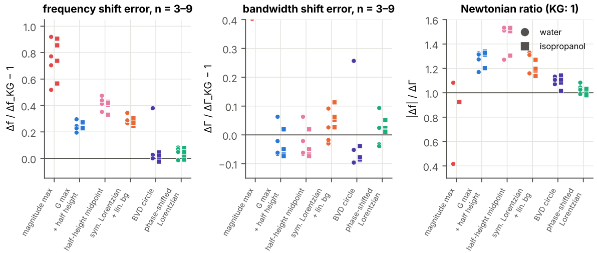
Figure 8: The three error metrics on overtones 3–9 (circles water, squares isopropanol) for six estimators.
