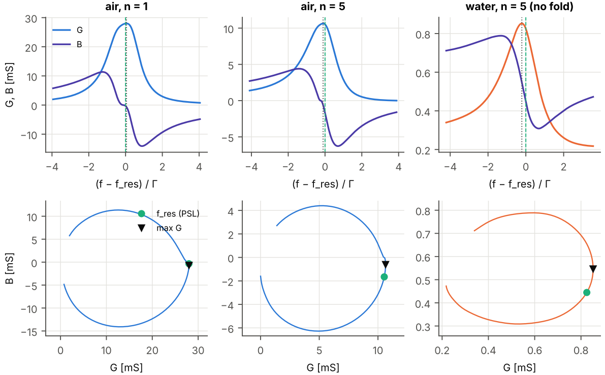
Figure 3: Reconstructed conductance and susceptance (top) and admittance locus (bottom) on \pm 4\Gamma around the resonance for the sweeps of Fig. 2. Dotted: the maximum of G ; dashed/marker: f_{\text{res}} from the phase-shifted Lorentzian. The maximum of G sits below f_{\text{res}} and the locus is rotated with respect to the G axis.
