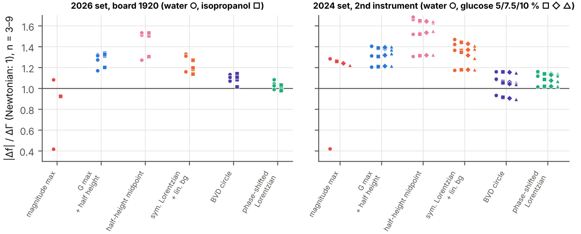
Figure 13: The Newtonian ratio on overtones 3–9 per estimator on the two instruments: board 1920 (water, isopropanol) and the instrument of 2024 (water and glucose 5, 7.5, 10 % w/v).
