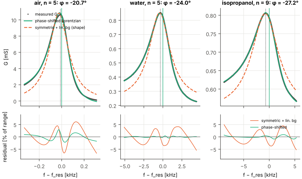
Figure 4: Conductance (dots) with the phase-shifted Lorentzian (solid) and the symmetric Lorentzian with linear background (dashed; drawn without its linear term) on \pm 3\Gamma_{\text{hh}} ; below, the residuals in percent of the range of G . Dotted vertical line: maximum of G ; solid: f_{\text{res}} of the phase-shifted fit.
