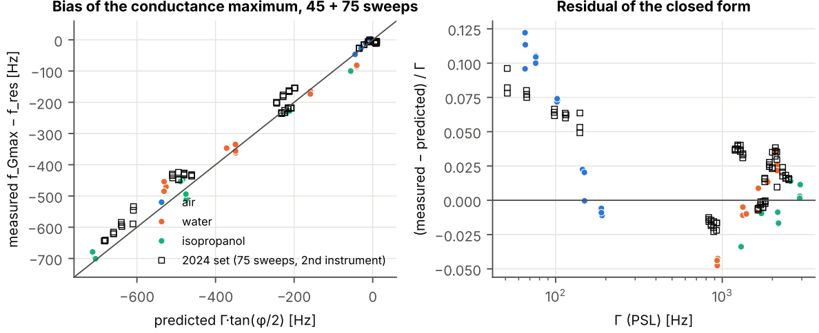
Figure 5: Left: measured f_{G_{\max}} - f_{\text{res}} against \Gamma \tan(\varphi/2) from the fit, 45 sweeps of 2026 (filled) and 75 sweeps of the second instrument (open squares); the line is the identity. Right: residual of the closed form in units of \Gamma .
