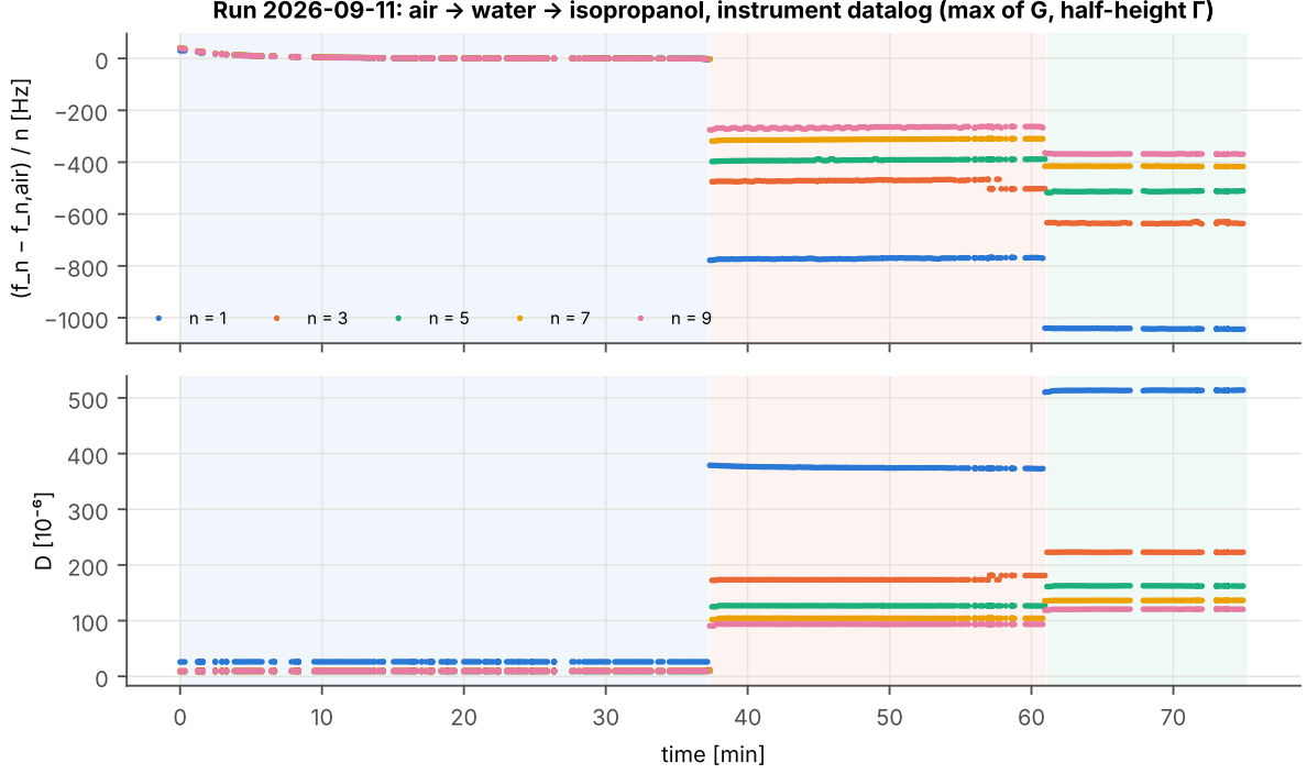
Figure 11: The run of 2026-09-11 as logged by the instrument (maximum of G , half-height \Gamma ): overtone-normalised frequency relative to the air value and dissipation factor against time; shaded: air, water, isopropanol.
