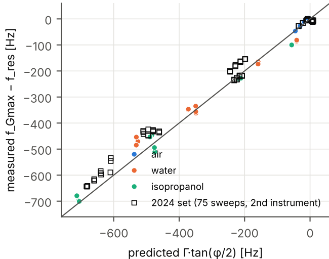
Bias of the conductance maximum, 45 + 75 sweeps
