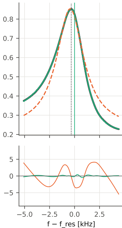
water, n = 5 : \phi = -24.0^\circ
