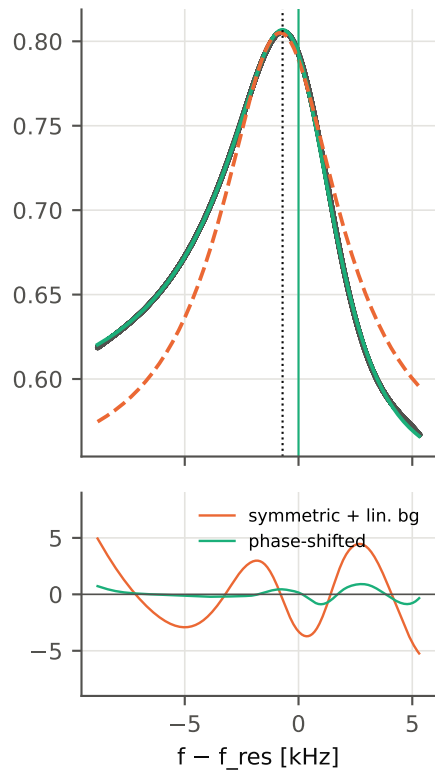
isopropanol, n = 9 : \phi = -27.2^\circ
