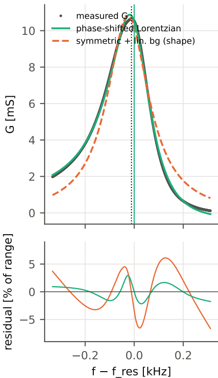
air, n = 5 : \phi = -20.7^\circ
