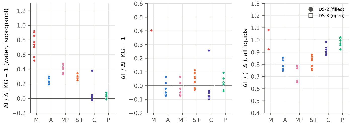
Error metrics on overtones 3-9 for six estimators; M: magnitude maximum, A: max G + half height, MP: midpoint, S+: symmetric + linear bg, C: BVD circle, P: phase-shifted Lorentzian
