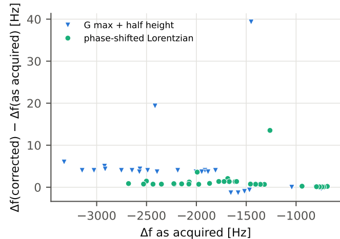
Effect of undoing the firmware carry-over (1/500 of the previous point) on the shifts, both datasets
