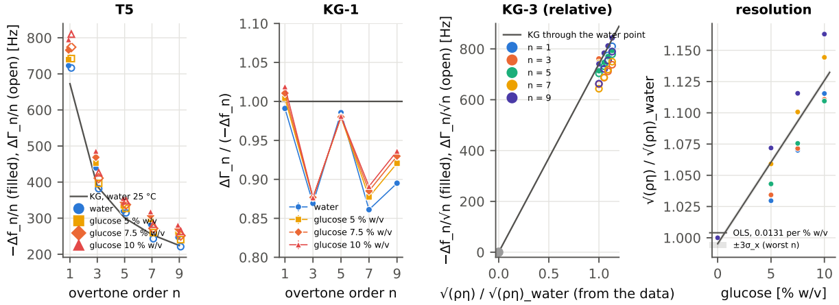
Figure 7: Experiment 3 (DS-3, estimator P). Template T5 for water and the three glucose solutions with the KG curve for water; KG-1 ratio against n ; KG-3 in relative units: -\Delta f_n/\sqrt{n} (filled) and \Delta \Gamma_n/\sqrt{n} (open) against the data-derived \sqrt{\rho\eta}/\sqrt{\rho\eta}_w , with the KG line through the water point; right: \sqrt{\rho\eta}/\sqrt{\rho\eta}_w against concentration per overtone with the least-squares line and the \pm 3\sigma noise band (worst overtone).
