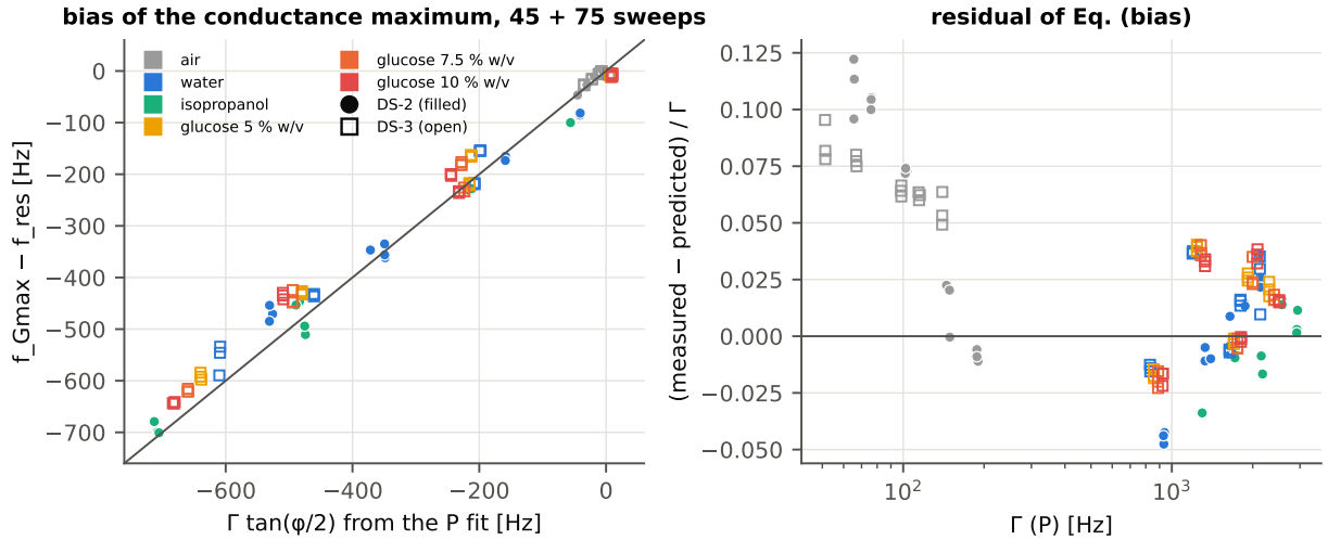
Figure 5: Left: measured f_{G\max} - f_{\text{res}} against \Gamma \tan(\varphi/2) from the fit, 45 sweeps of DS-2 (filled) and 75 of DS-3 (open), coloured by medium; line: identity. Right: residual of Eq. (9) in units of \Gamma .
