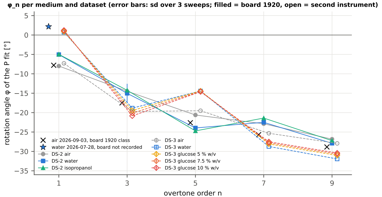
Figure 8: The rotation angle of the fit against the overtone order for every medium and dataset: DS-2 (filled, board 1920: air, water, isopropanol), DS-3 (open, second instrument: air, water, glucose 5, 7.5, 10 % w/v), the air sweeps of 2026-09-03 (crosses) and the water sweep of 2026-07-28 on an unrecorded board (star). Error bars: sd over three sweeps.
