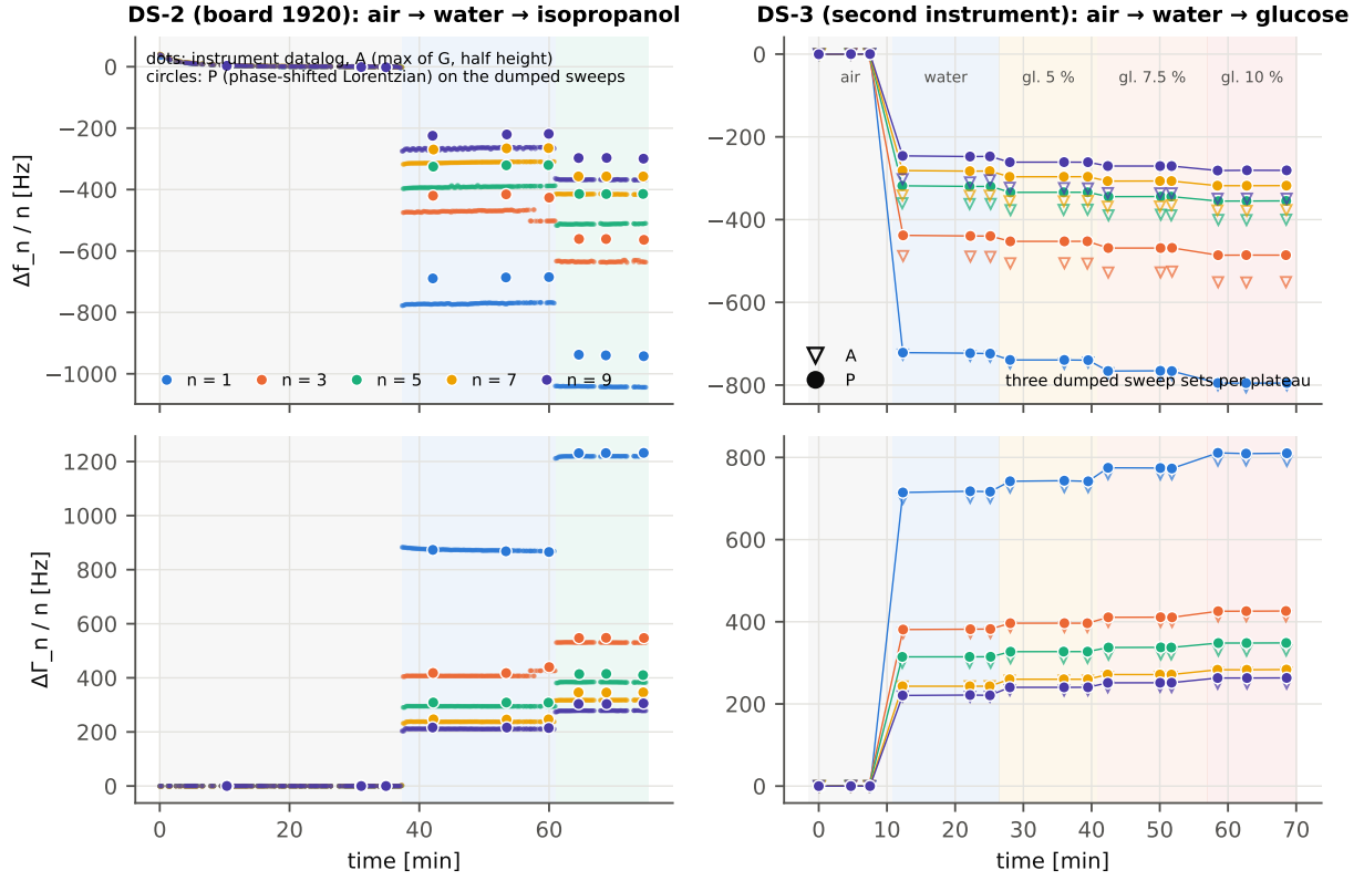
Figure 3: Template T4: overtone-normalised shifts against time, \Delta f_n/n (top) and \Delta \Gamma_n/n (bottom), one colour per overtone, relative to the air plateau. Left: DS-2, the instrument datalog (estimator A, live) with the P values of the dumped sweeps as circles. Right: DS-3, the dumped sweeps only (A open triangles, P filled circles). Shaded: air, water, isopropanol / glucose plateaus.
