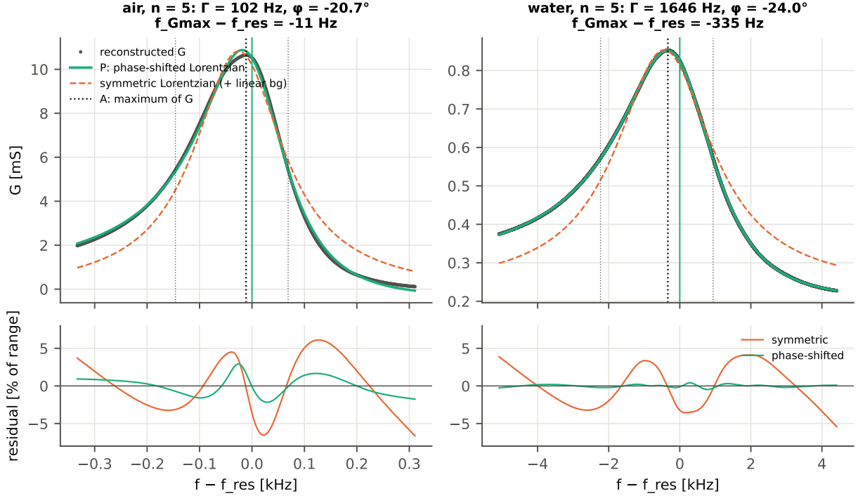
Figure 2: Reconstructed conductance of the 5th overtone in air (left) and water (right), board 1920, with the phase-shifted Lorentzian (solid), the symmetric Lorentzian with linear background (dashed, drawn without its linear term), the maximum of G and its half-height crossings (dotted) and f_{\text{res}} of the fit (solid vertical); below, the residuals in percent of the range of G .
