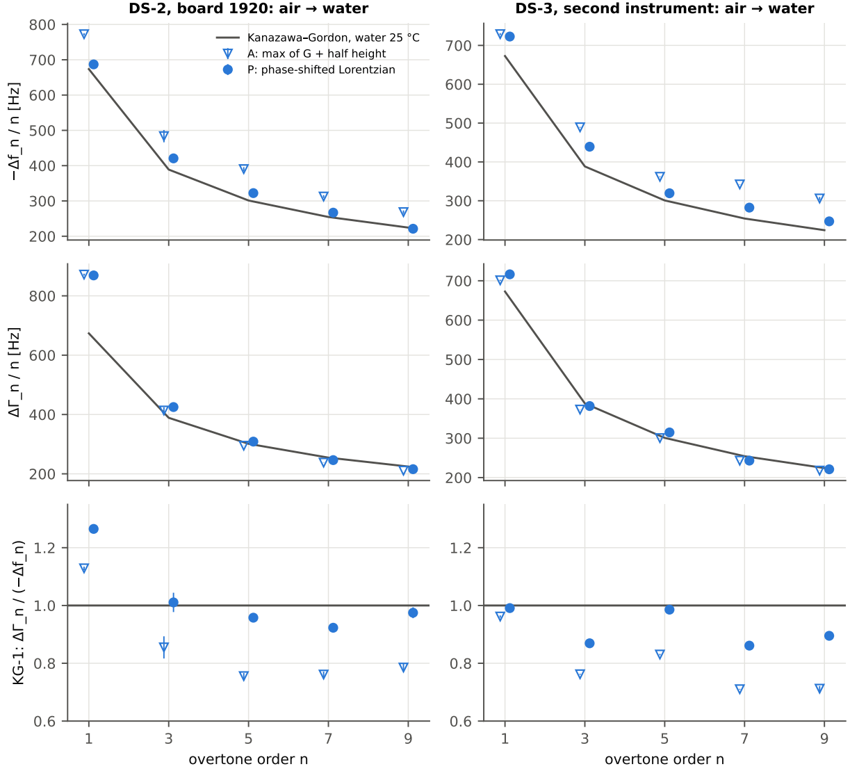
Figure 4: Template T5 and KG-1 for the air \rightarrow water step of DS-2 (left) and DS-3 (right): -\Delta f_n/n , \Delta \Gamma_n/n and r_n = \Delta \Gamma_n/(-\Delta f_n) against the overtone order for A (open triangles) and P (filled circles), with the Kanazawa-Gordon prediction for water at 25 °C. Error bars: replica scatter.
