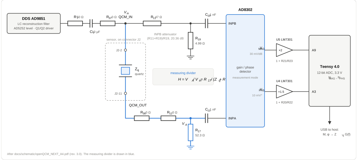
Figure 1: Measurement circuit: the quartz sensor in a divider with R_{17} , read by the AD8302 gain/phase detector (drawn after the openQCM NEXT schematic).
