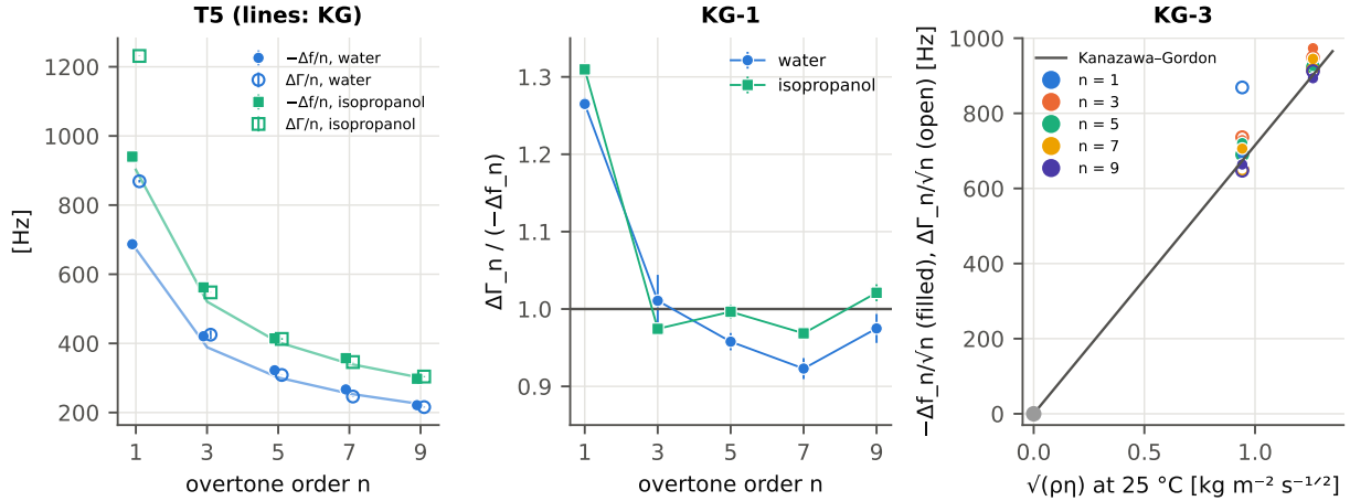
Figure 6: Experiment 2 (DS-2, estimator P). Left, template T5: -\Delta f_n/n (filled) and \Delta\Gamma_n/n (open) for water and isopropanol with the KG curves. Centre, KG-1: r_n against n . Right, KG-3: -\Delta f_n/\sqrt{n} (filled) and \Delta\Gamma_n/\sqrt{n} (open) against the tabulated \sqrt{\rho\eta} of air (origin), water and isopropanol at 25 °C, one colour per overtone, with the KG line of slope f_F^{3/2}/\sqrt{\pi\rho_q\mu_q} .
