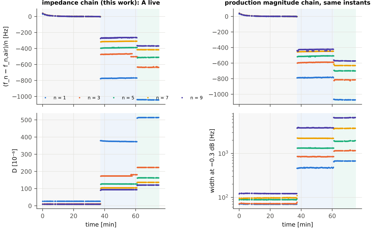
Figure 8: The run of 2026-09-11 as logged by the instrument: the impedance chain (left; A live) and the production magnitude chain at the same instants (right); overtone-normalised frequency relative to the air plateau, dissipation factor, and the production -0.3 dB width.
