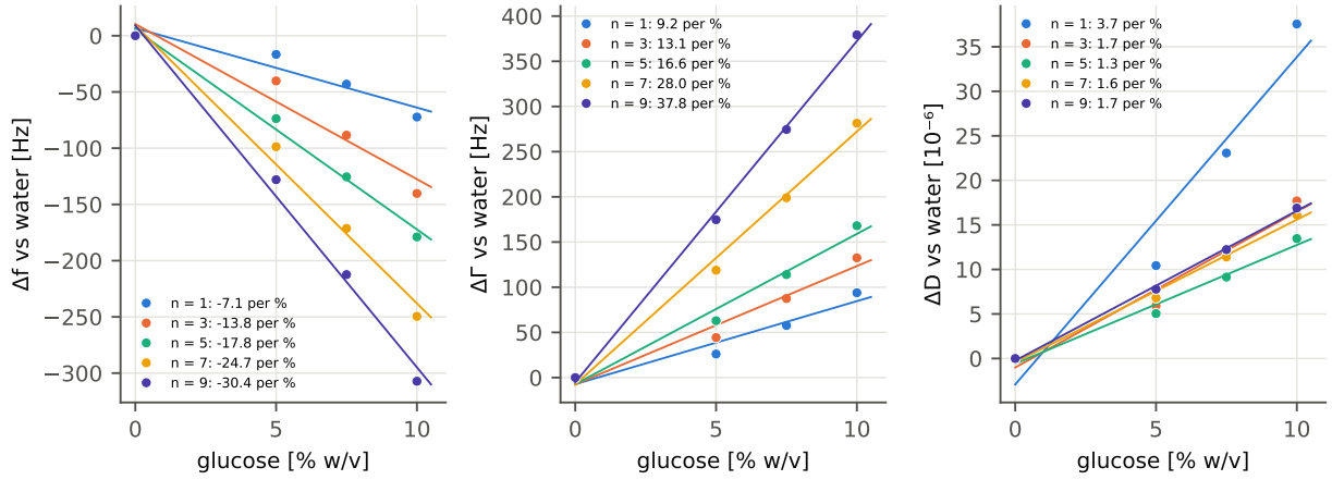
Figure 9: Shifts relative to water of the fitted resonance frequency, half-bandwidth and dissipation against glucose concentration, one line per overtone (least squares with intercept).
