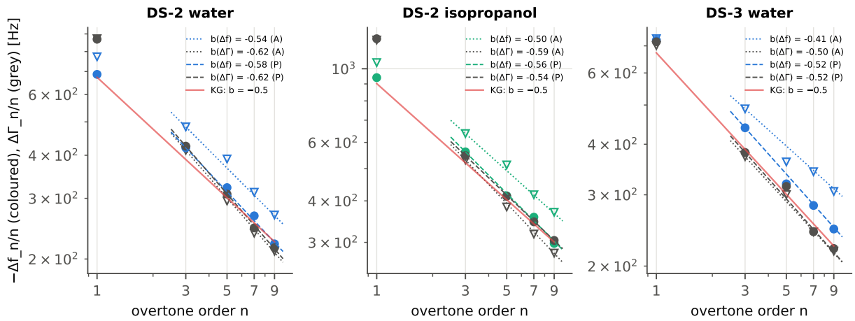
Figure 12: KG-2 on log-log axes: -\Delta f_n/n and \Delta \Gamma_n/n against n for A and P with the fitted slopes on n = 3-9 and the KG line of slope -1/2 .
