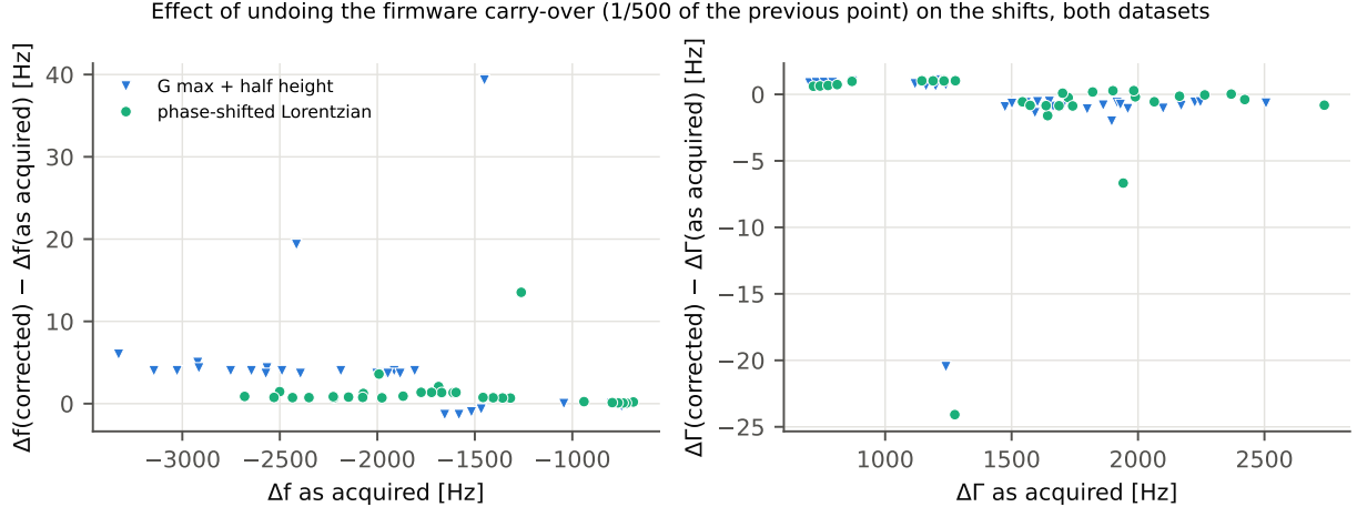
Figure 6: Difference of the air-to-liquid shifts between the firmware-corrected and the as-acquired variants, both datasets, estimators A and P.
