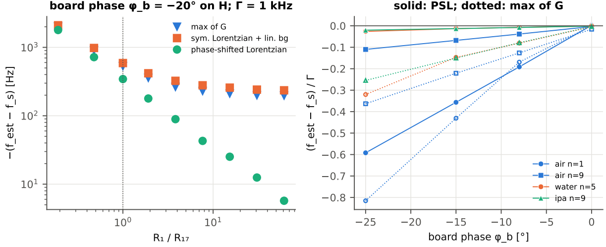
Figure 5: Forward model. Left: error of three estimators against R_1/R_{17} for a board phase of -20^\circ on the transfer function ( \Gamma = 1 kHz). Right: error in units of \Gamma against the board phase for four measured-like cases; solid: phase-shifted fit; dotted: maximum of G .
