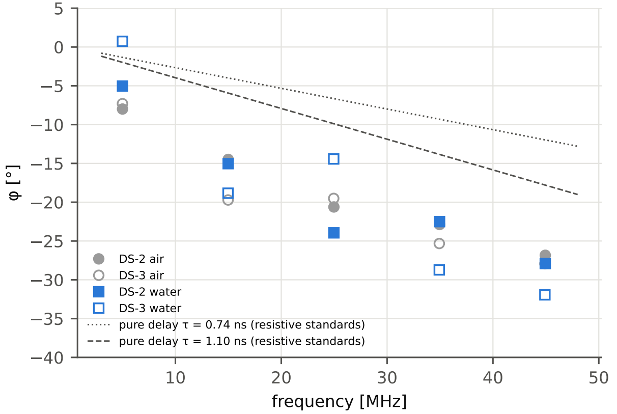
Figure 11: The rotation angle against frequency for air and water on both instruments, with the phase of a pure delay for the two delays measured on the resistive standards of board 1920.
