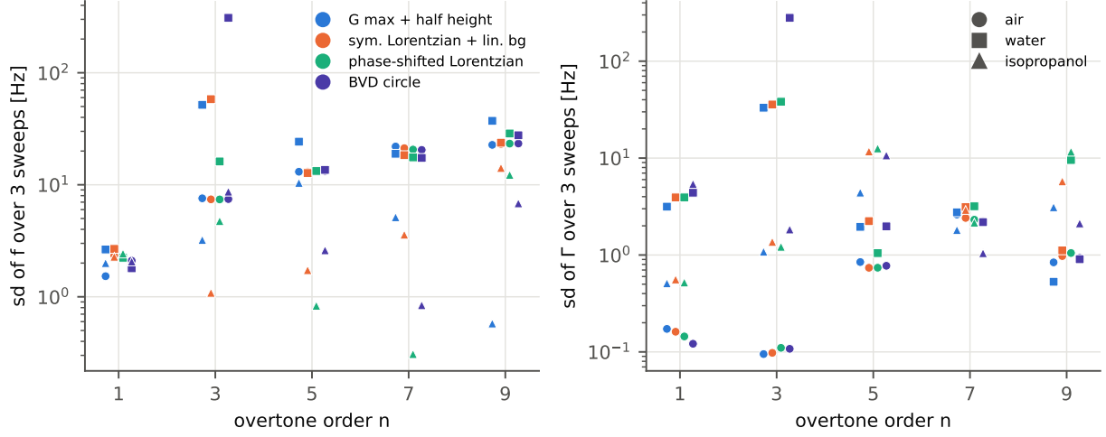
Figure 4: Standard deviation over the three plateau sweeps of f_{\text{res}} (left) and \Gamma (right) per estimator, overtone and load, DS-2.
