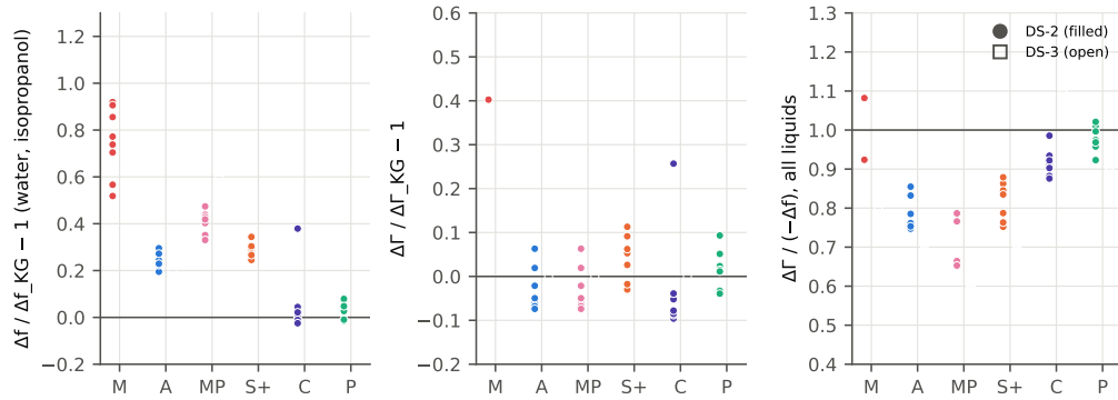
Figure 7: Error metrics on overtones 3–9 for six estimators on both datasets: \epsilon_f , \epsilon_\Gamma (water and isopropanol) and r_n (all liquids).
