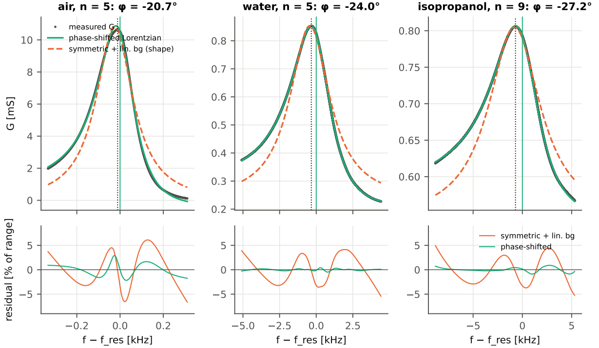
Figure 3: Conductance (dots) with the phase-shifted Lorentzian (solid) and the symmetric Lorentzian with linear background (dashed) on \pm 3 \Gamma_{\text{hh}} for three sweeps of DS-2; below, the residuals in percent of the range of G .
