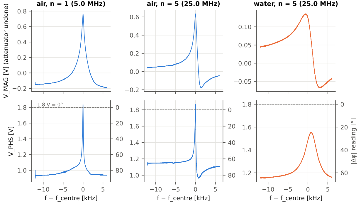
Figure 1: Raw detector voltages for the fundamental and the 5th overtone in air and for the 5th overtone in water (DS-2). Right axis: the unsigned phase reading. In air the reading folds at zero and overshoots it (the signature of \delta ); in water it does not reach zero.
