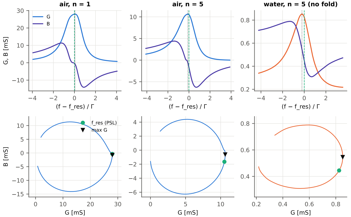
Figure 2: Reconstructed conductance and susceptance (top) and admittance locus (bottom) on \pm 4 \Gamma for the sweeps of Fig. S1. Dotted: the maximum of G ; marker: f_{\text{res}} of the phase-shifted fit.
