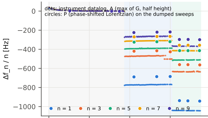
DS-2 (board 1920): air → water → isopropanol
