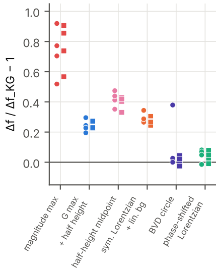
frequency shift error, n = 3-9
