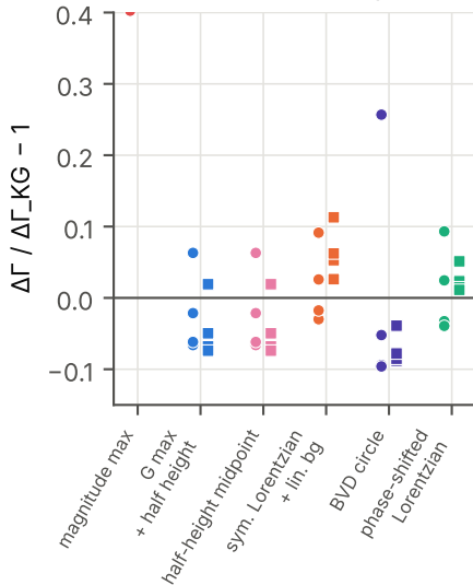
bandwidth shift error, n = 3-9
