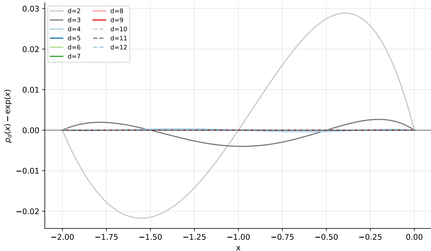
Chebyshev-Lobatto approximation error on [-2.0, 0.0]
