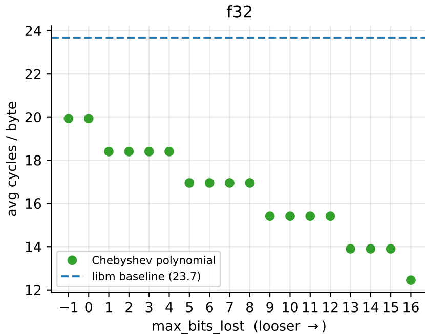
Accuracy vs performance Pareto for our polynomial approximation of \exp(x)
