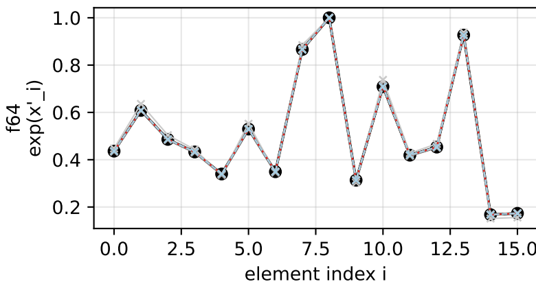
seed=0, N=16
