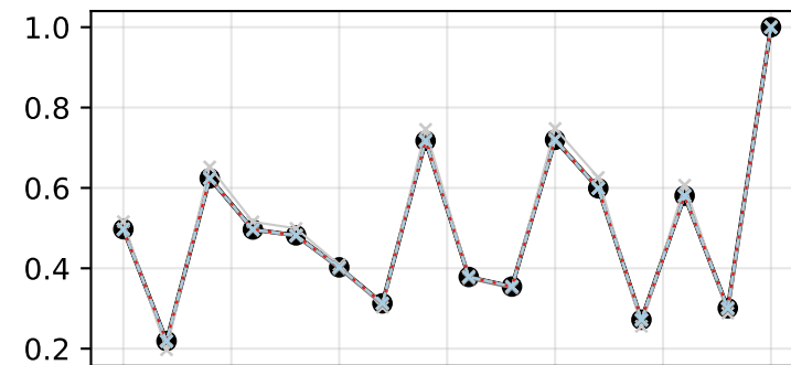
seed=2, N=16
