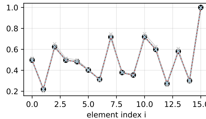
seed=2, N=16
