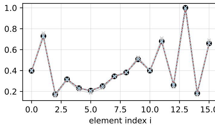
seed=1, N=16
