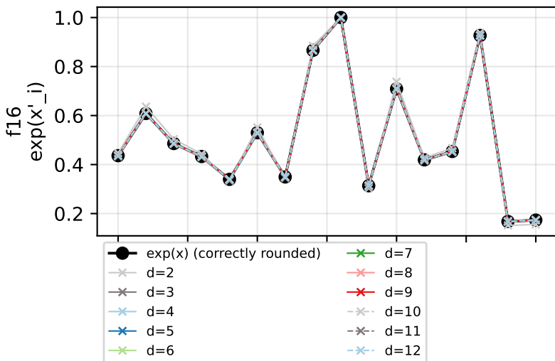
seed=0, N=16
