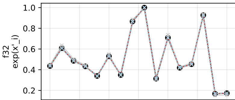
seed=0, N=16
