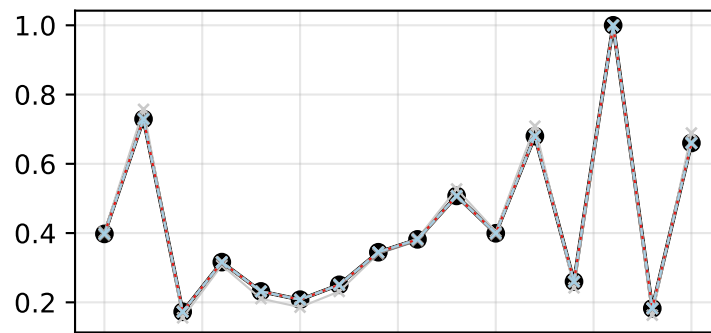
seed=1, N=16
