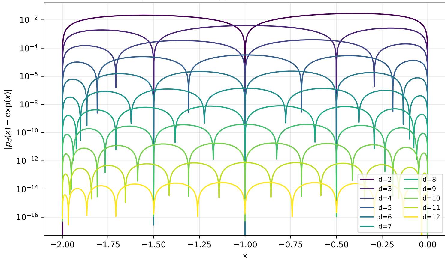
Chebyshev-Lobatto approximation error on [-2.0, 0.0]
