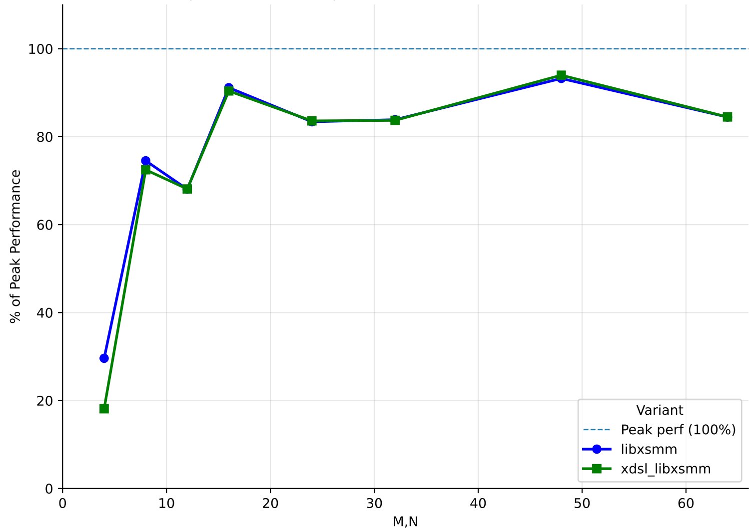
Performance of square matrix multiplication kernels, for M = N , K = 16 and 1 \leq M, N \leq 64
