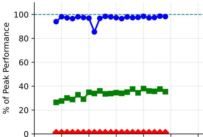
(c) N = K = 128 , f32, Intel Skylake
