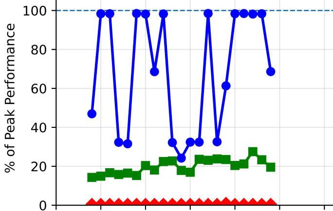
(c) N = K = 128 , f32, Intel Skylake
