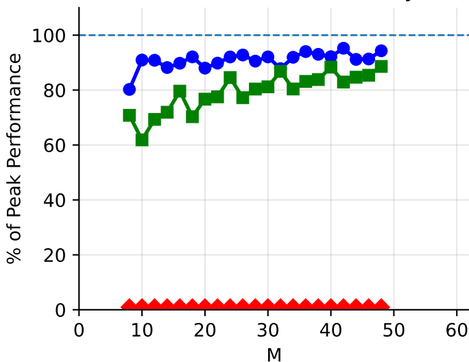
(c) N = K = 128 , f32, Intel Skylake
