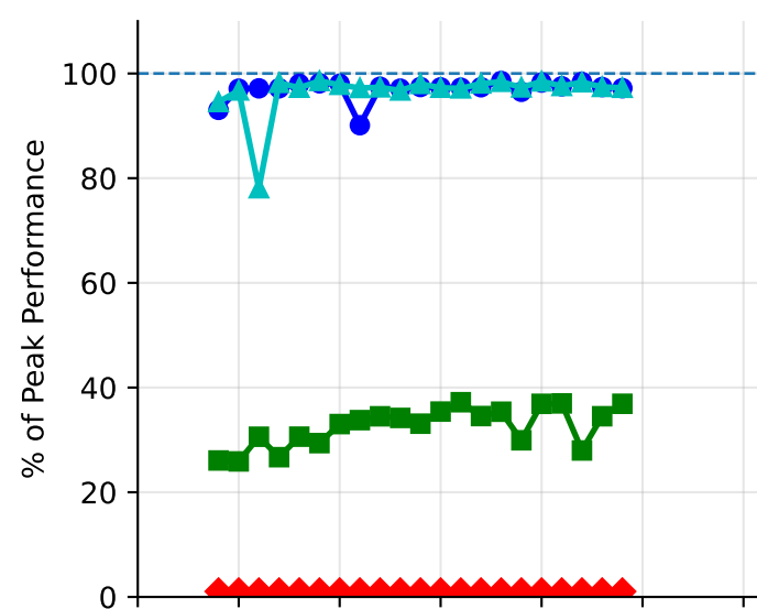
(a) N = K = 128 , f32 , AMD Zen 5
