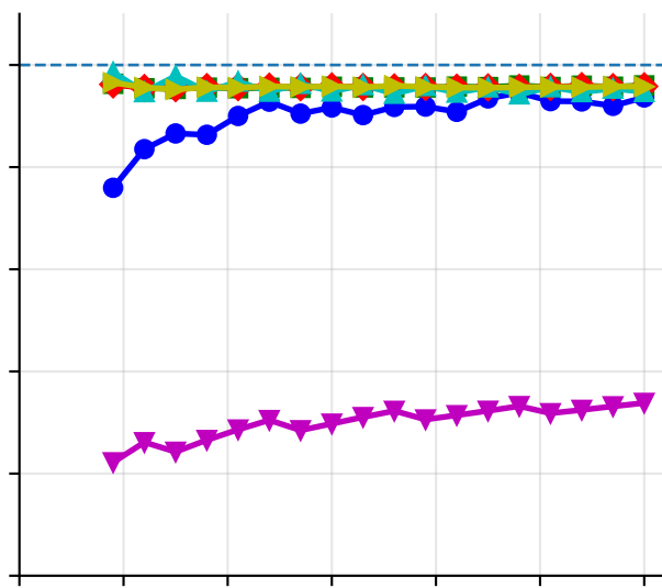
(b) M = K = 64, f64, AMD Zen 5
