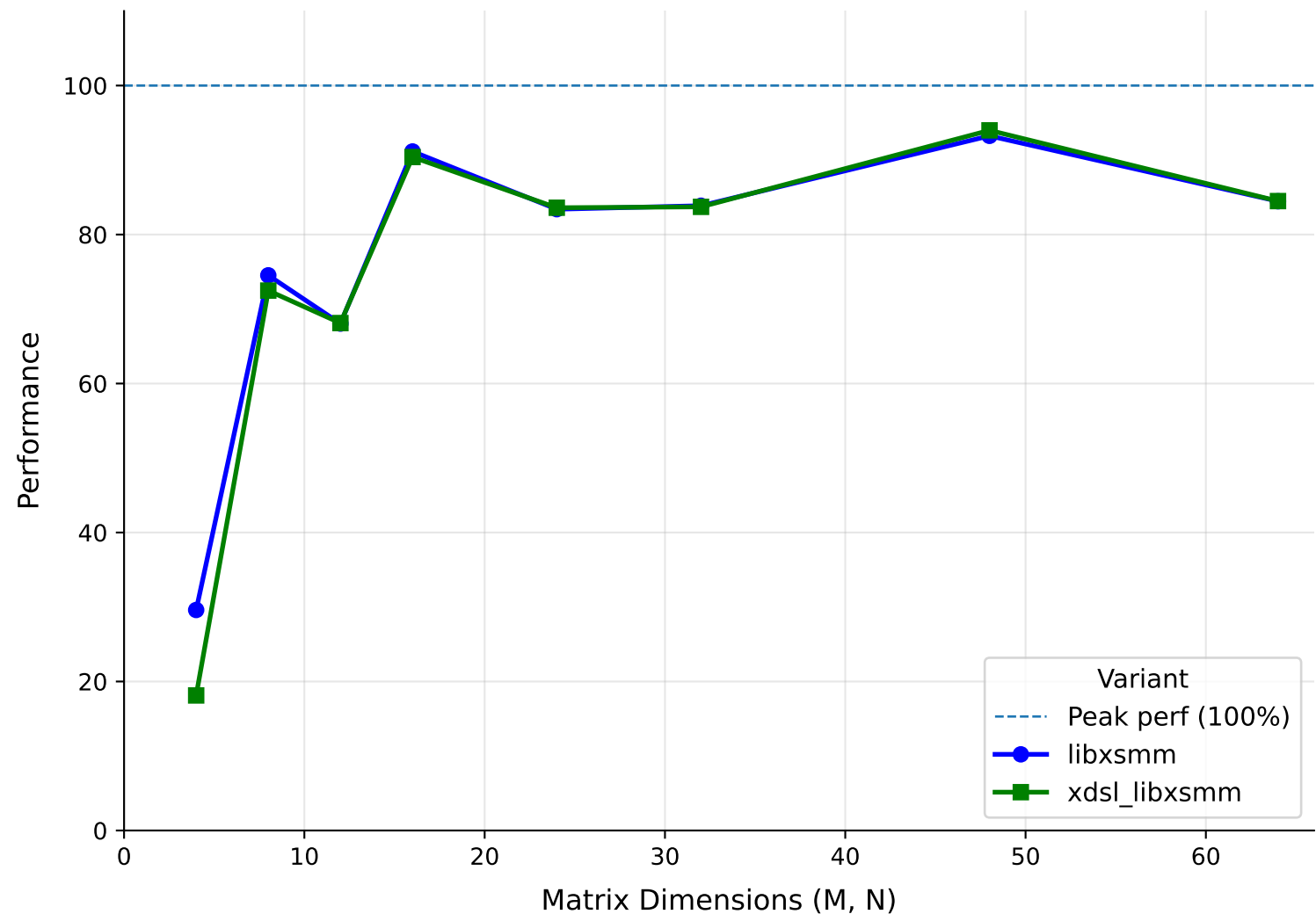
Performance of Square F64 Kernels ( M = N , K = 16 )
