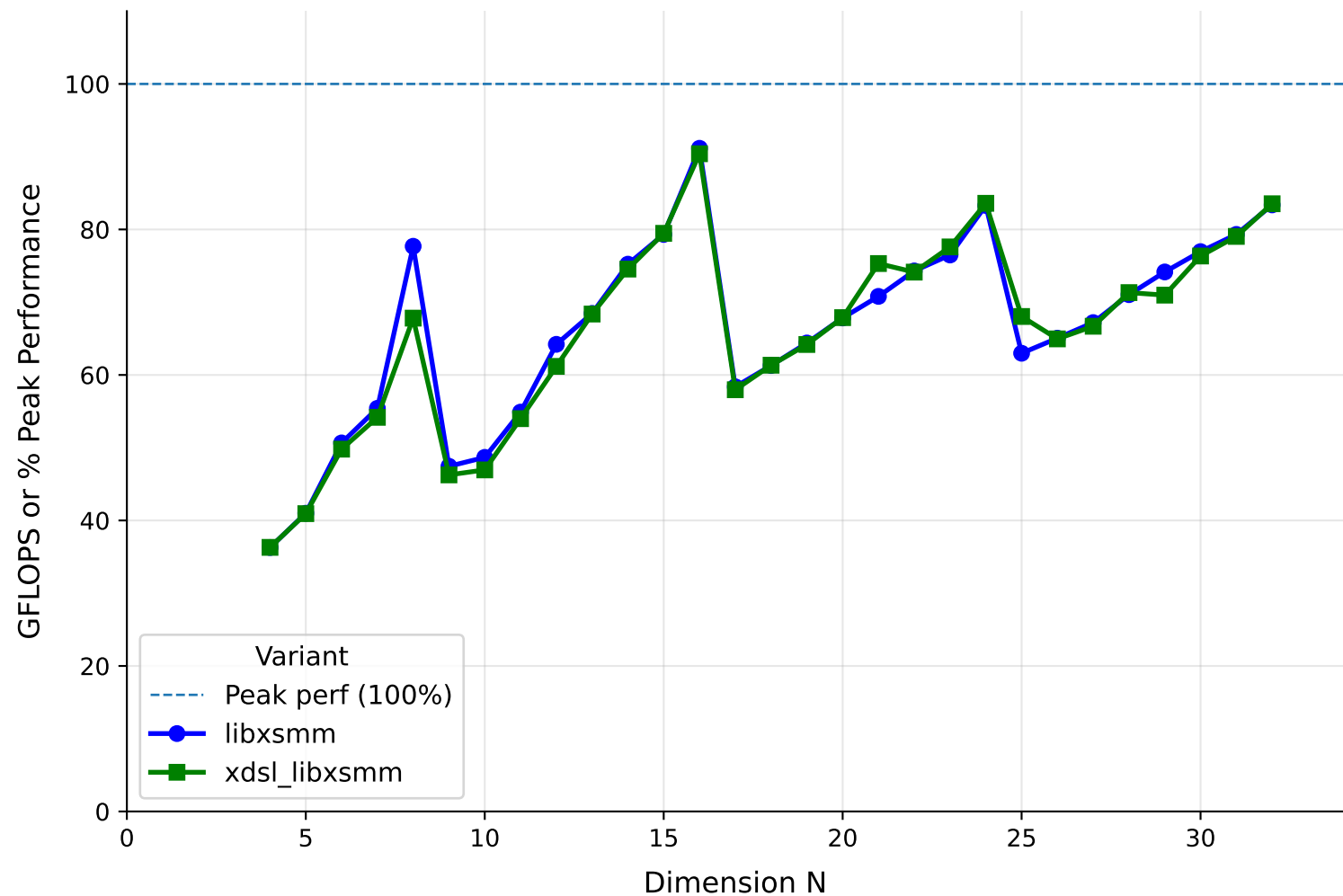
Performance of F64 Kernels M = 16, K = 16 (continuous sweep)
