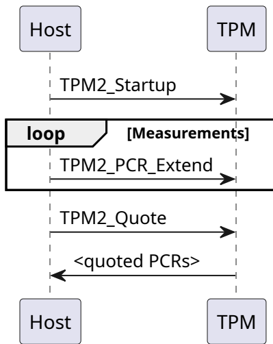
Figure 4: Startup Sequence (UML)
