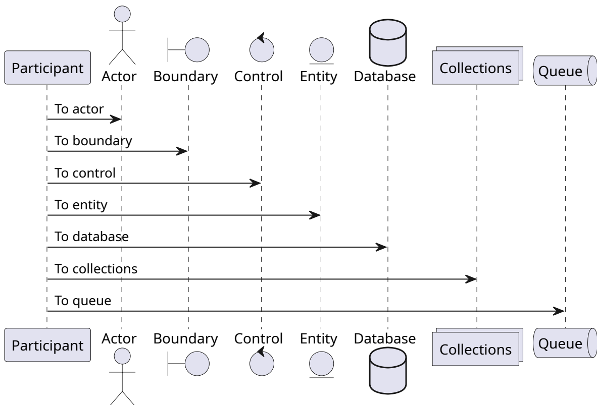
Figure 5: Included UML
