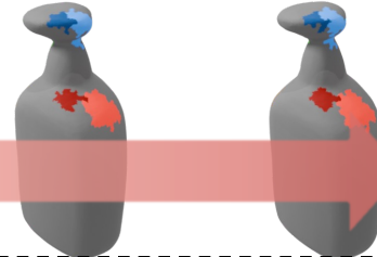
Pose Refinement
