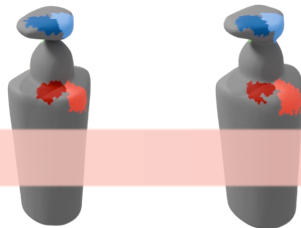
Shape Interpolation
