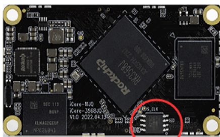
3 SPI Nor
