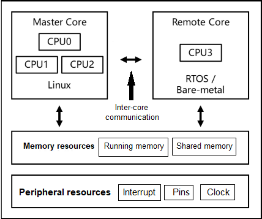
Figure 4-1-1 Linux+RTOS/Bare-metal system architecture
