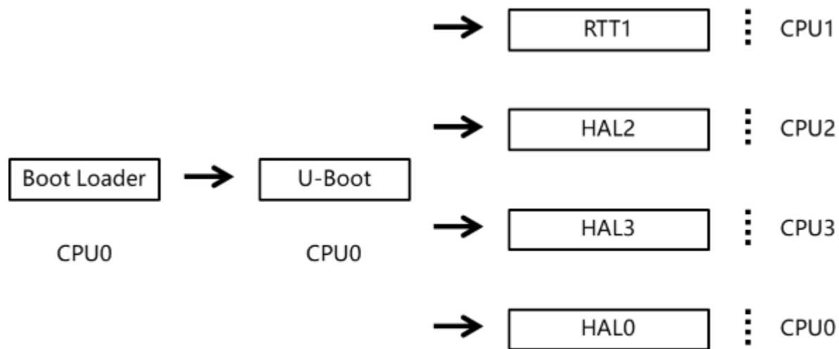
Figure 5-1-5 rtt + hal + hal + hal
