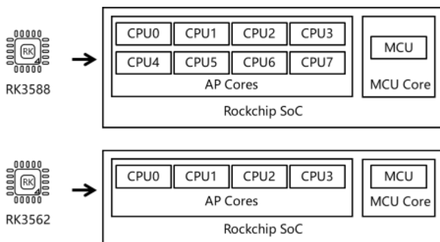
Figure 5-1-1 Rockchip SoC architecture
