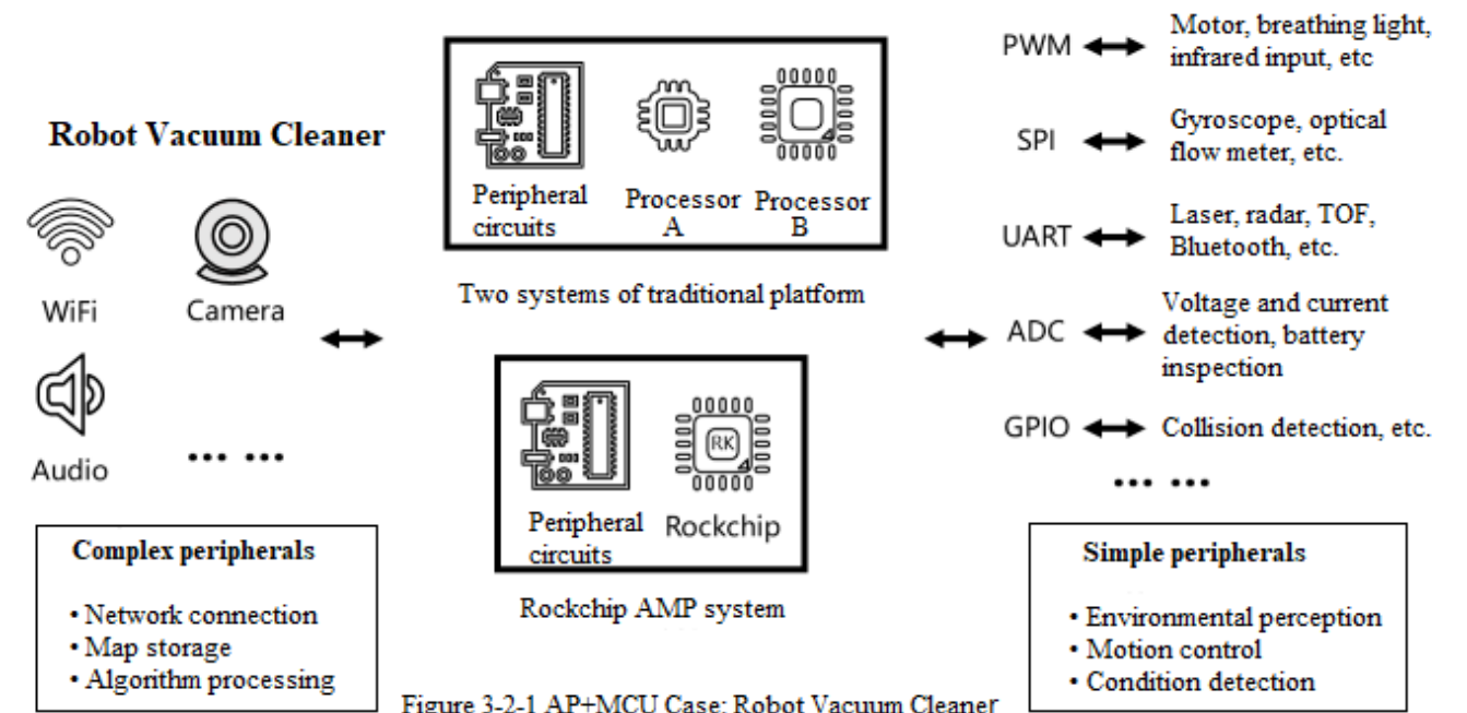
Figure 3-2-1 AP+MCU Case: Robot Vacuum Cleaner
