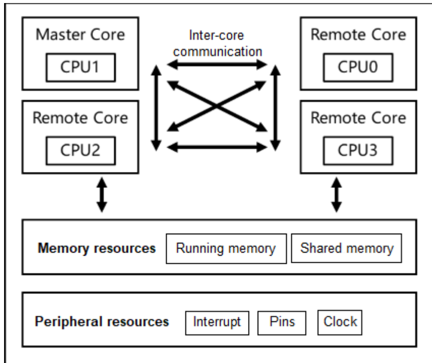
Figure 4-1-2 RTOS+Bare-metal system architecture
