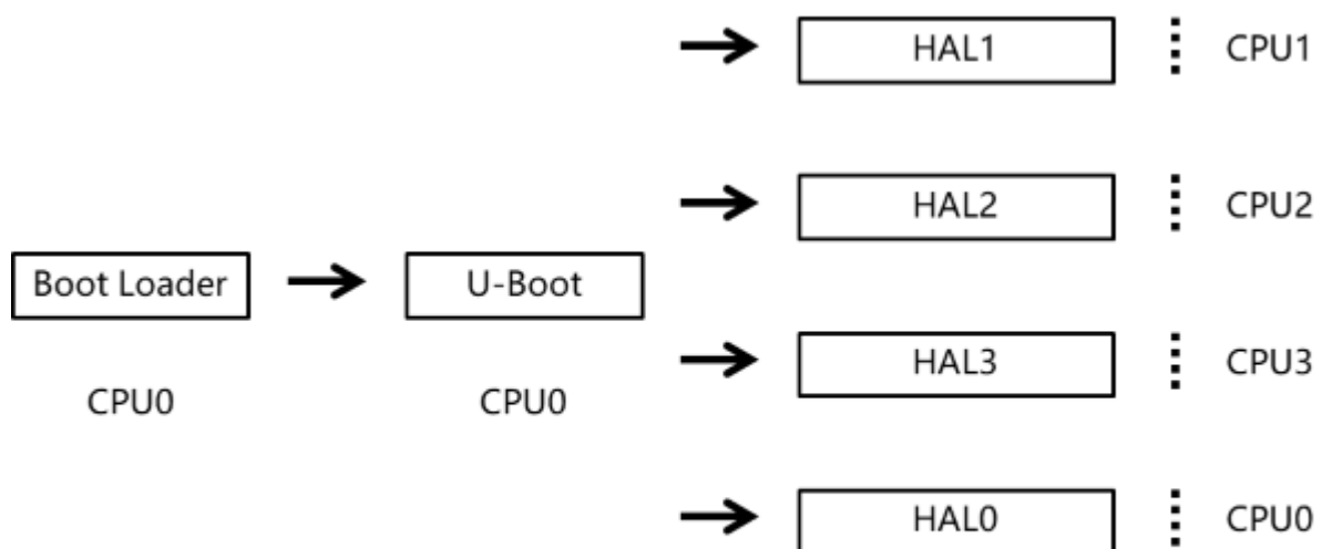
Figure 5-1-4 hal + hal + hal + hal
