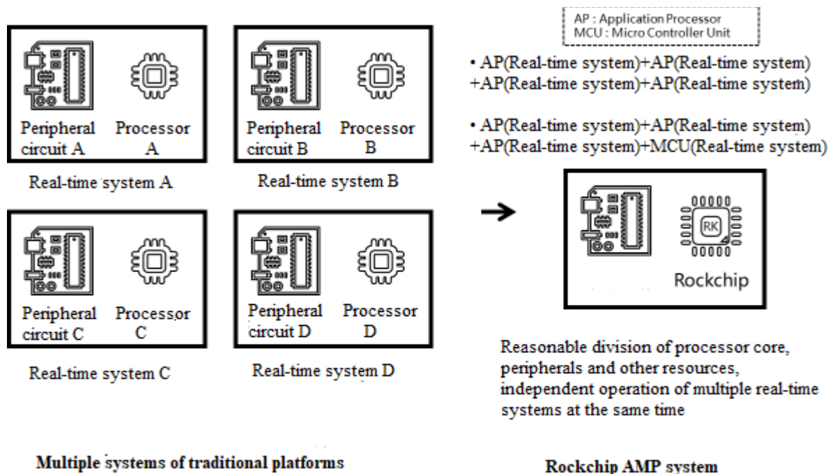
Figure 1-1-2 Independent operation of multiple real-time systems at the same time
