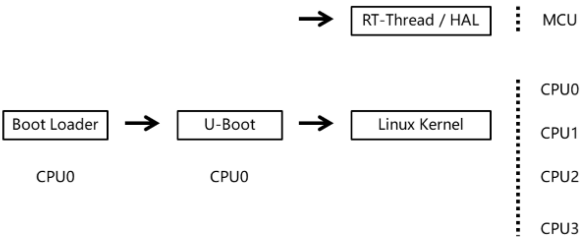
Figure 5-1-6 kernel + mcu rtt / hal
