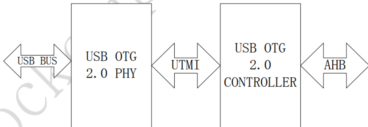
Figure 1-2 USB 2.0 OTG Block Diagram
