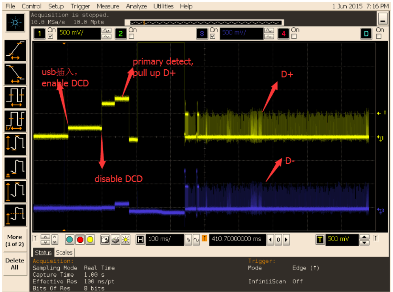
Figure 8-2 SDP detection signals
