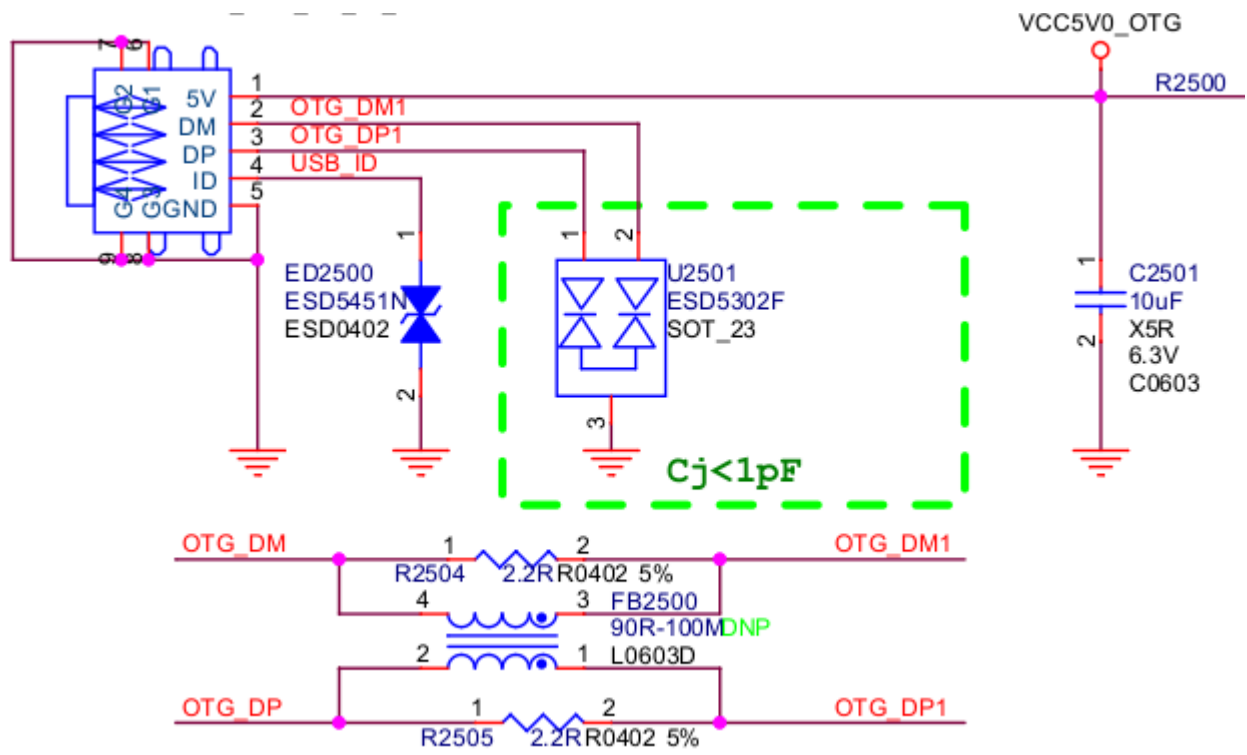
Figure 2-6 USB 2.0 OTG Micro-Interface
