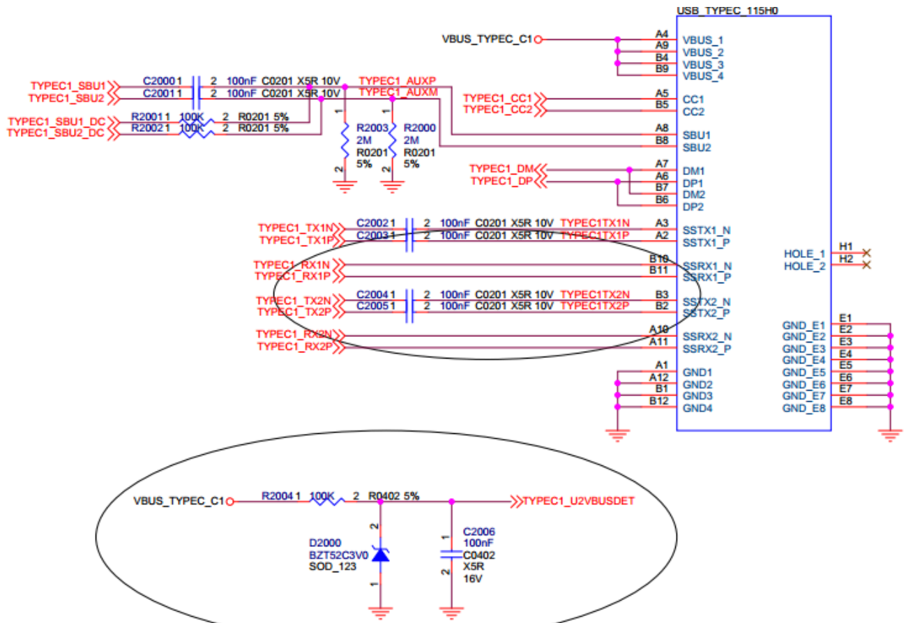
Figure 2-11 USB 3.0 OTG Type-C interface
