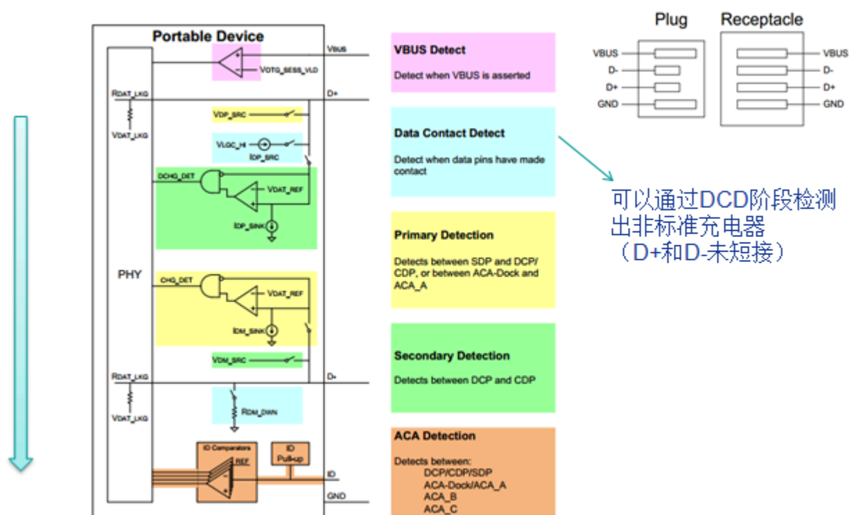
Figure 8-1 USB Charging Detection Process
