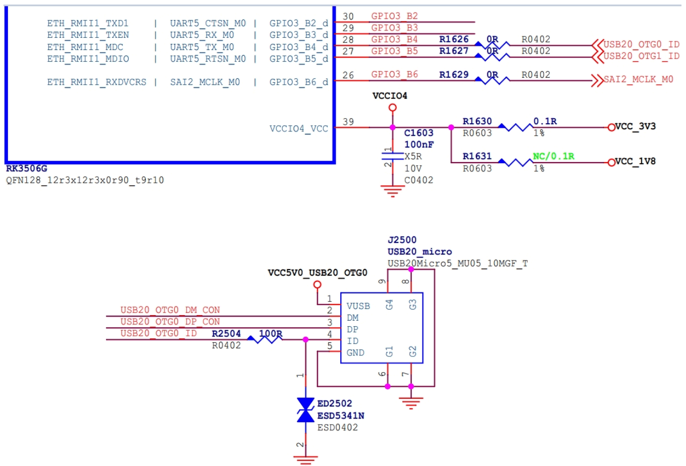
Figure 2-16 USB OTG ID GPIO Hardware Circuit Diagram
