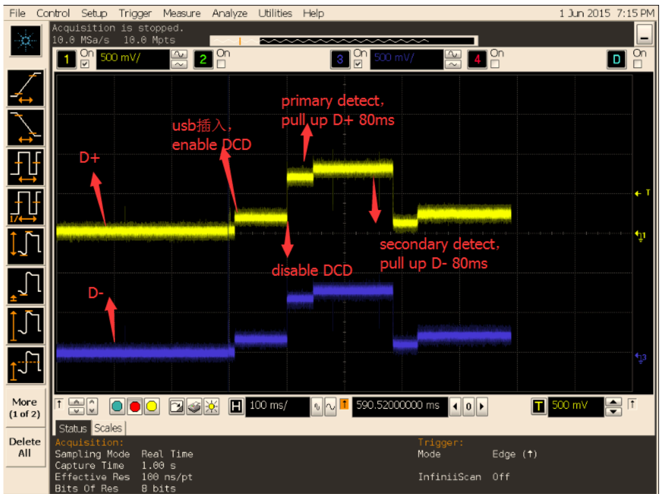
Figure 8-3 DCP detection signals
