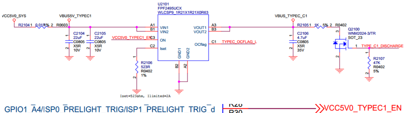
Figure 2-13 USB 3.0 VBUS Control Circuit-1 (Control by GPIO)
