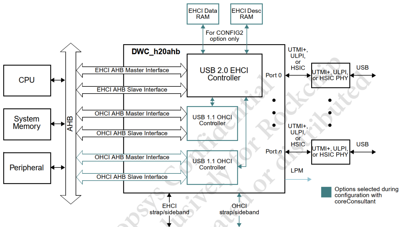
Figure 5-4 EHCI & OHCI controller system-level block diagram
