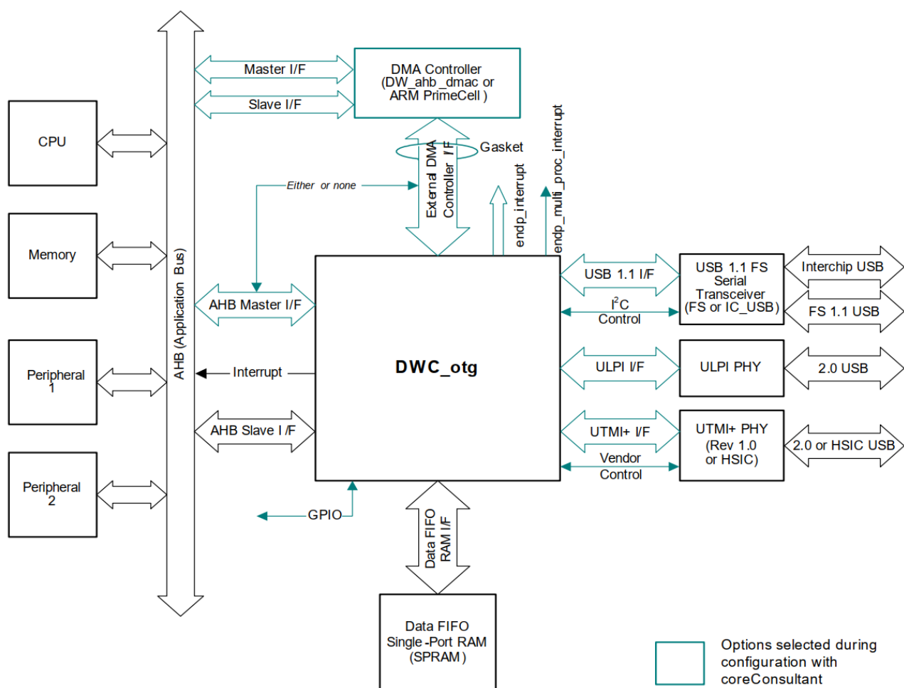
Figure 5-2 DWC2 controller system-level block diagram
