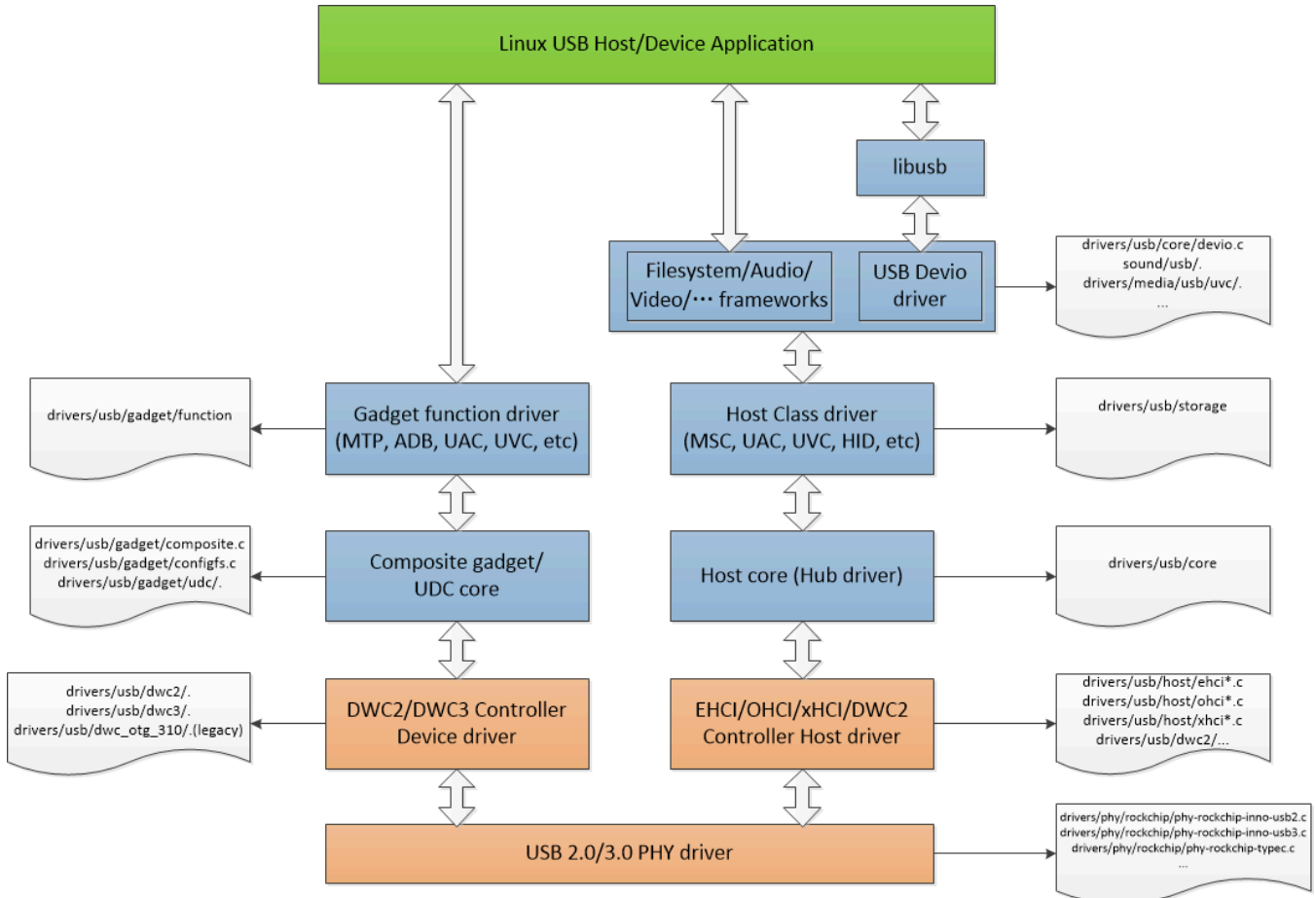
Figure 5-1 Linux USB driver framework
