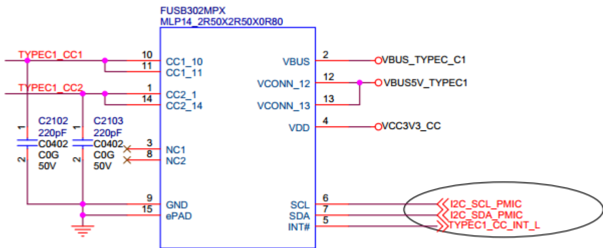
Figure 2-11 USB 3.0 OTG Type-C interface
