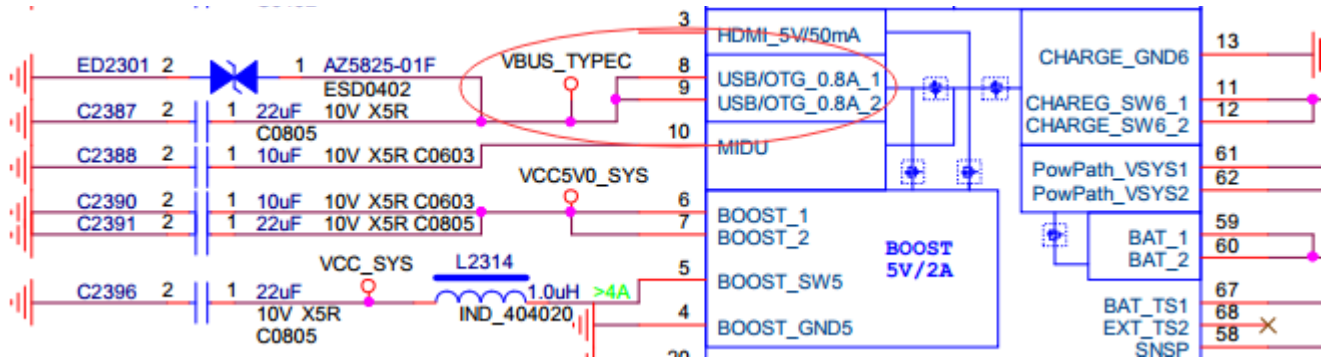
Figure 2-14 USB 3.0 VBUS Control-2 (Control by RK818)
