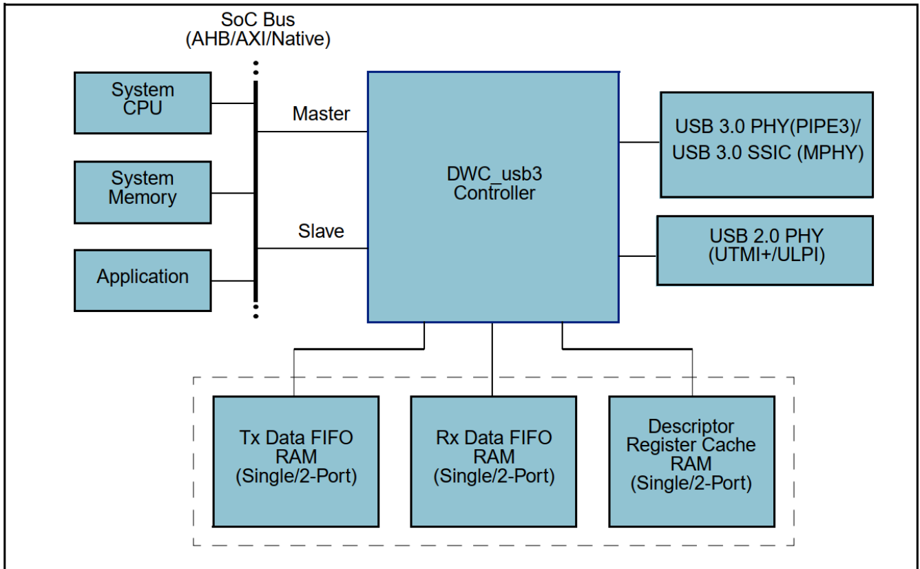
Figure 5-5 DWC3 controller system-level block diagram
