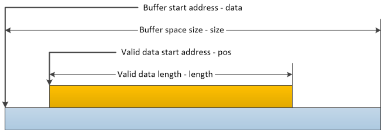
Figure 6 Important parameter description of MppPacket
