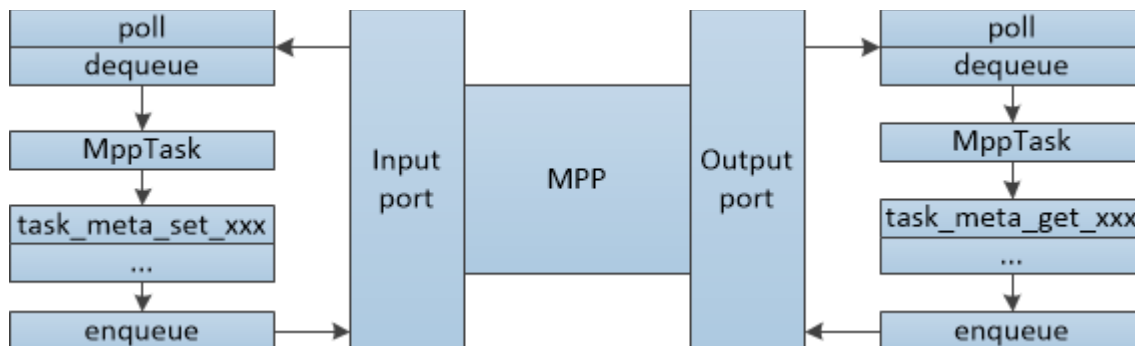
Figure 8 Use MppTask for input and output
