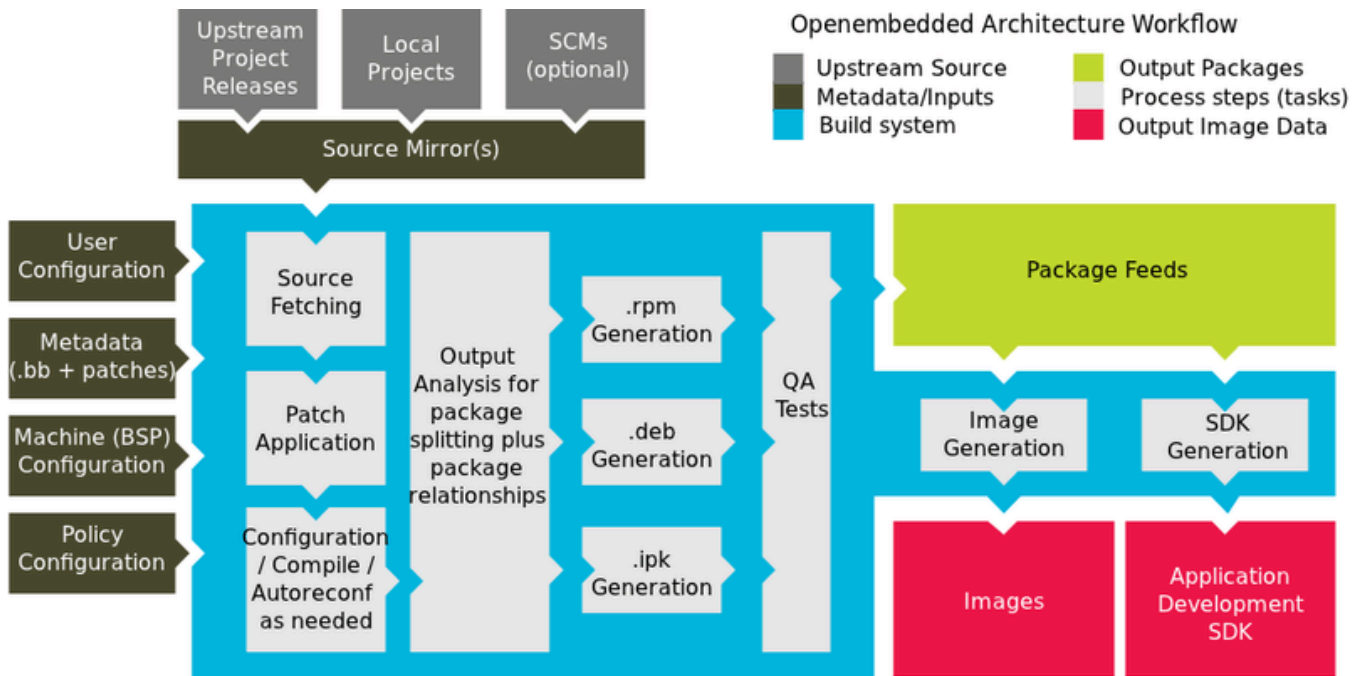
Figure 2-1 Yocto Compilation block diagram
