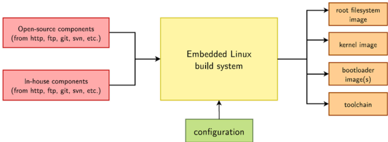
Figure 1-1 Buildroot Compilation Block Diagram
